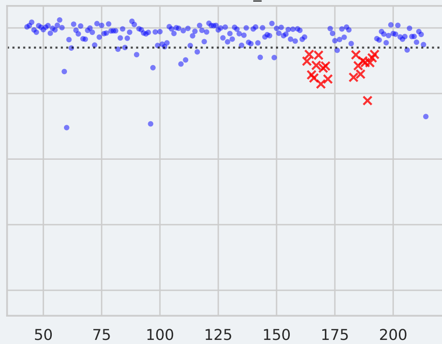
Feature: DST_PORT
