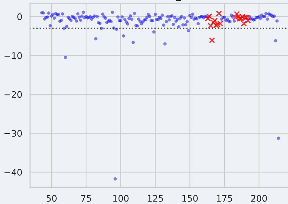
Feature: SRC_PORT
