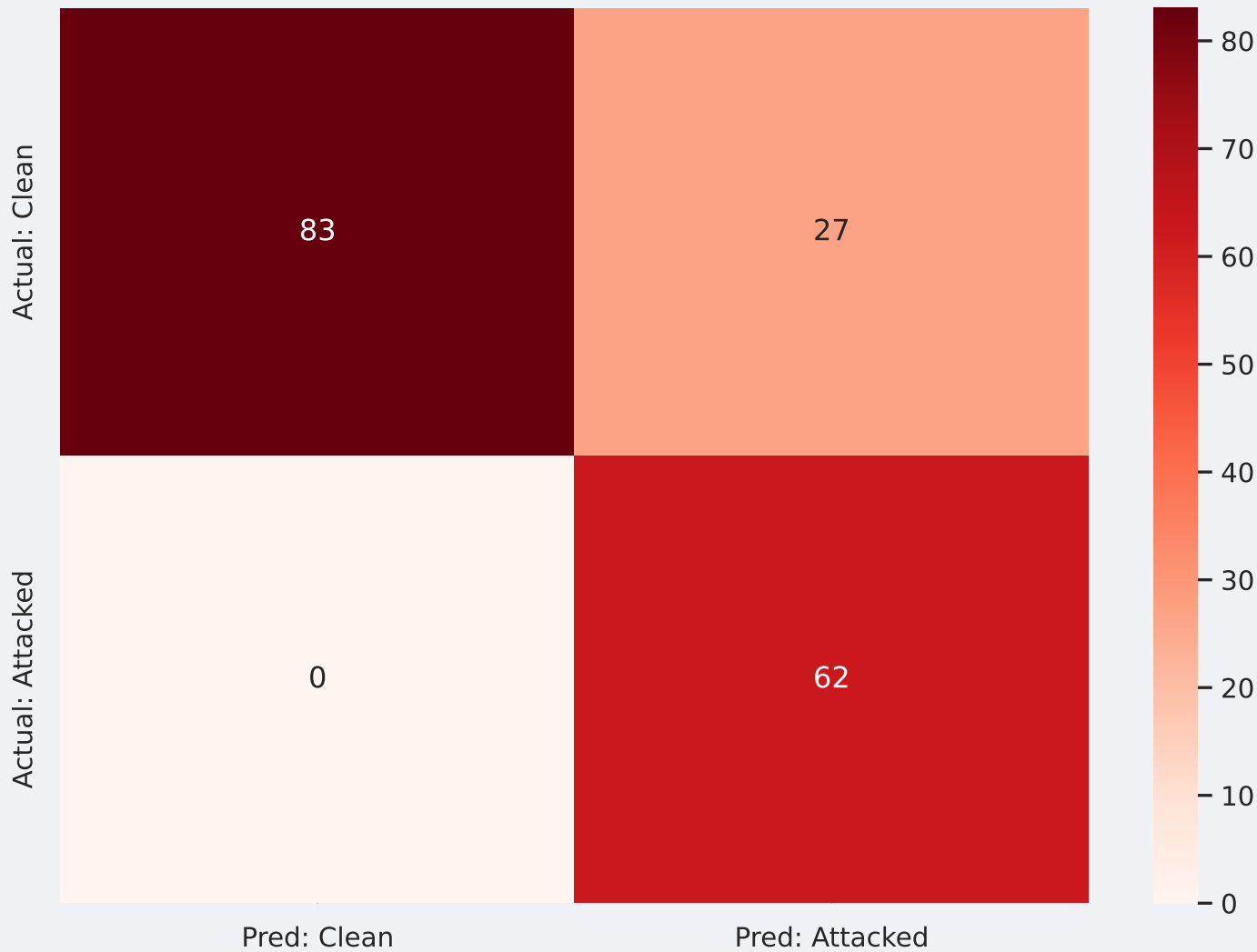
Confusion Matrix
