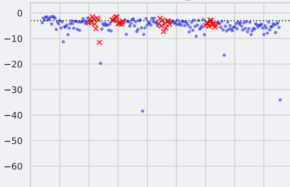
Feature: SRC_IP
