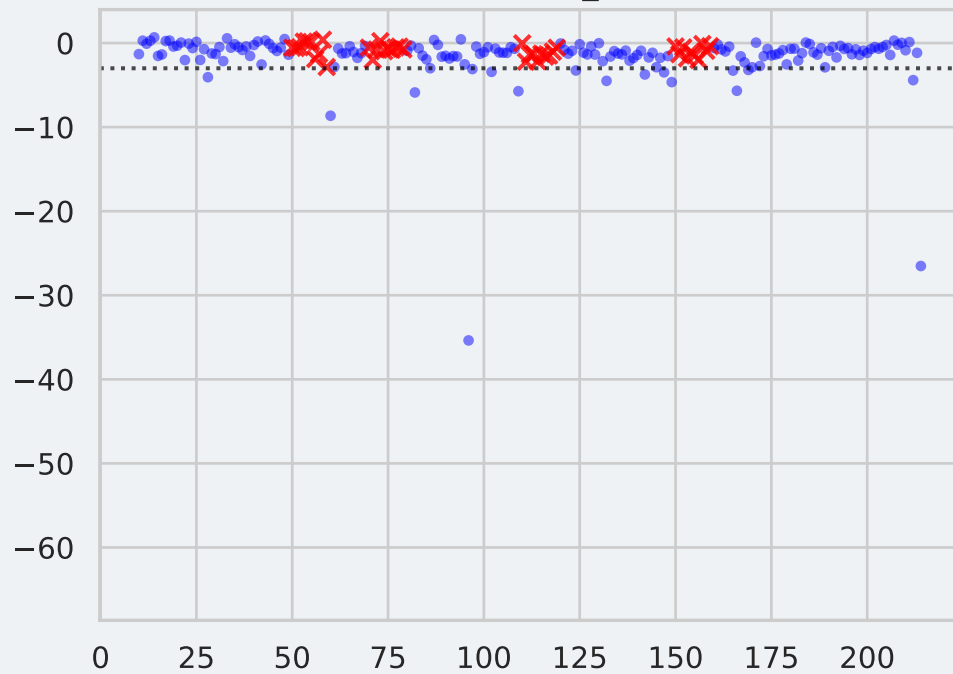
Feature: SRC_PORT
