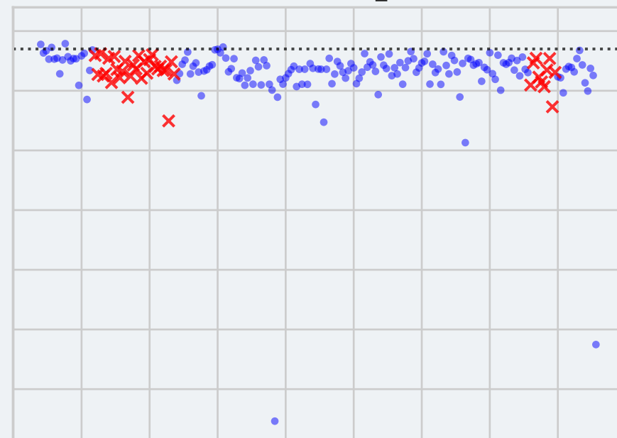
Feature: DST_PORT
