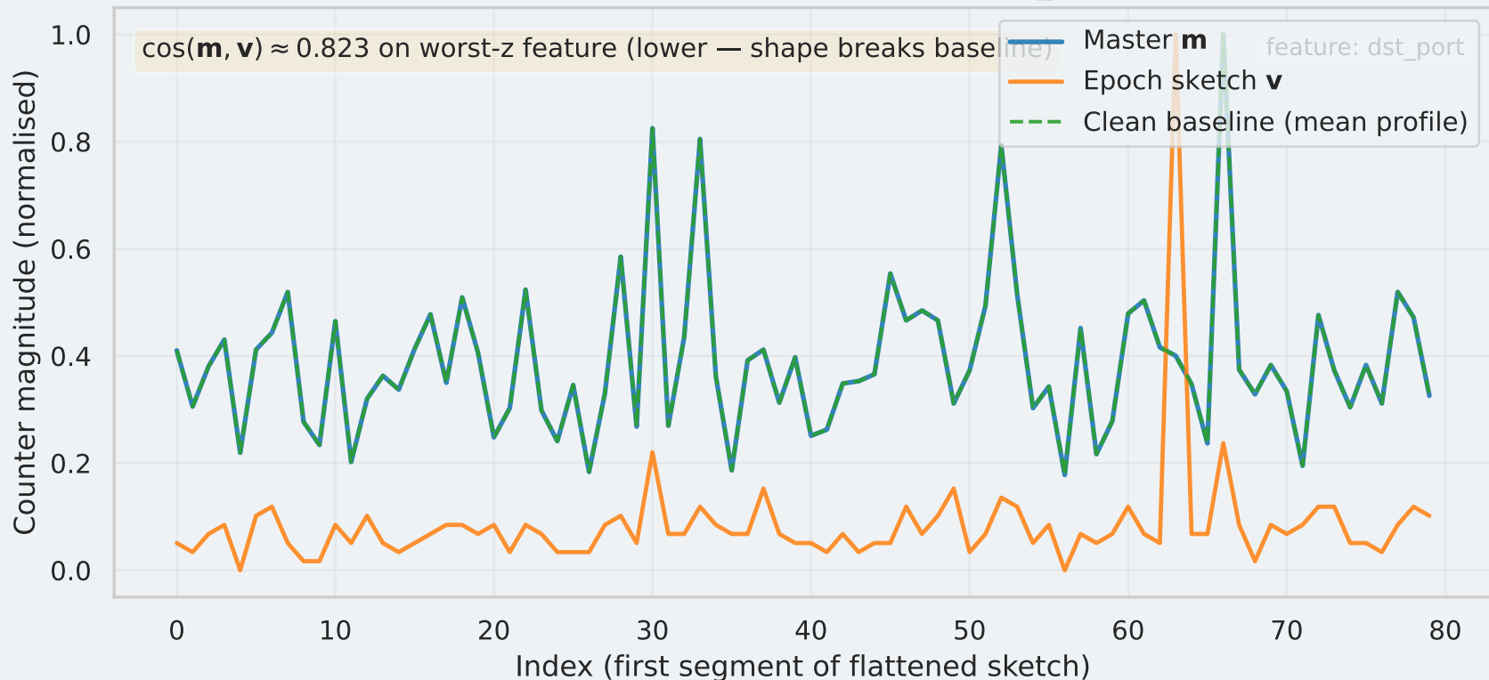
Attack epoch vs master (epoch 189 epoch_000189)
