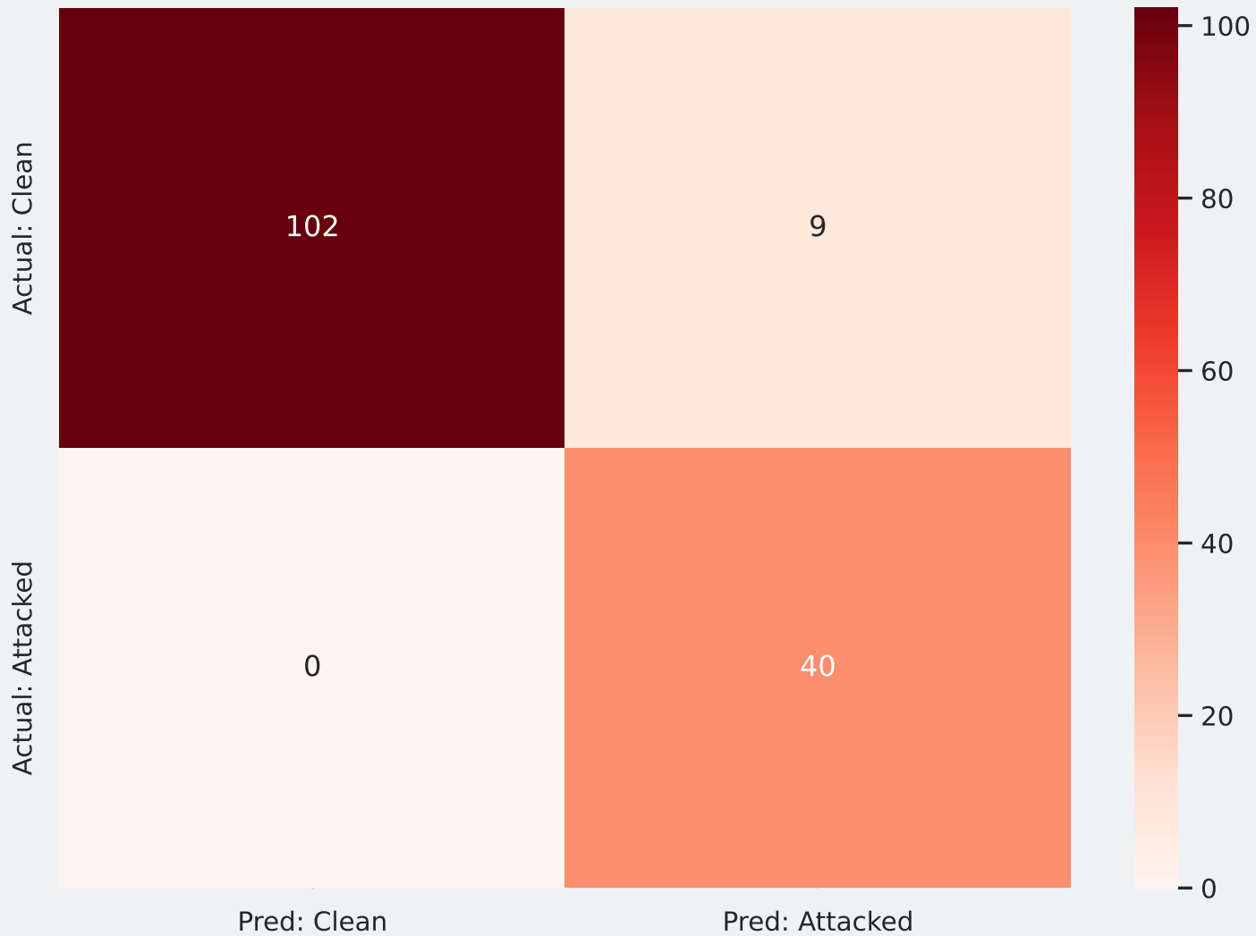
Confusion Matrix
