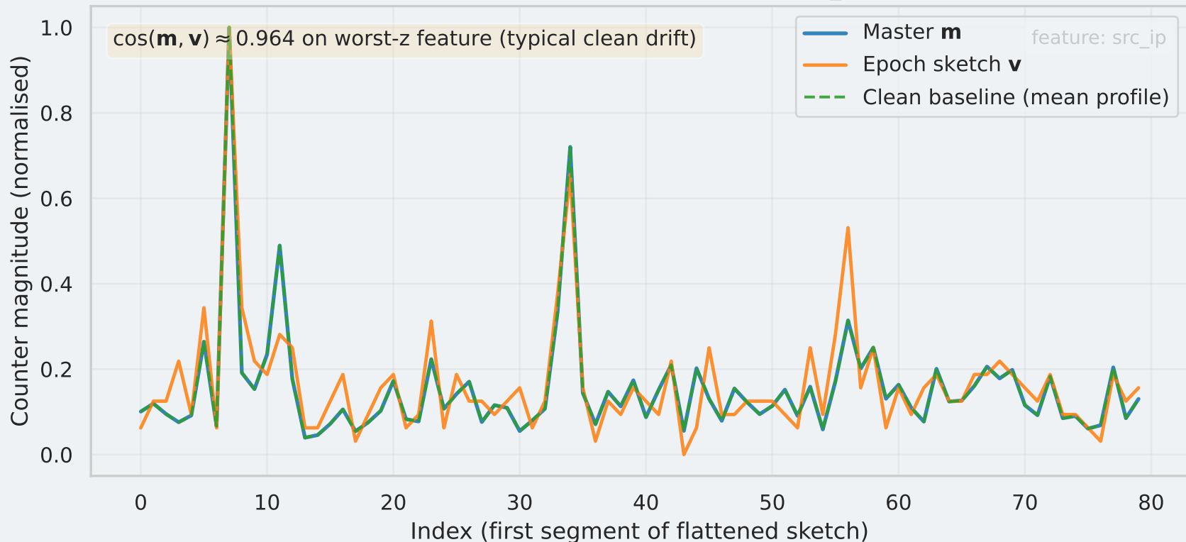
Benign epoch vs master (epoch 152 epoch_000152)
