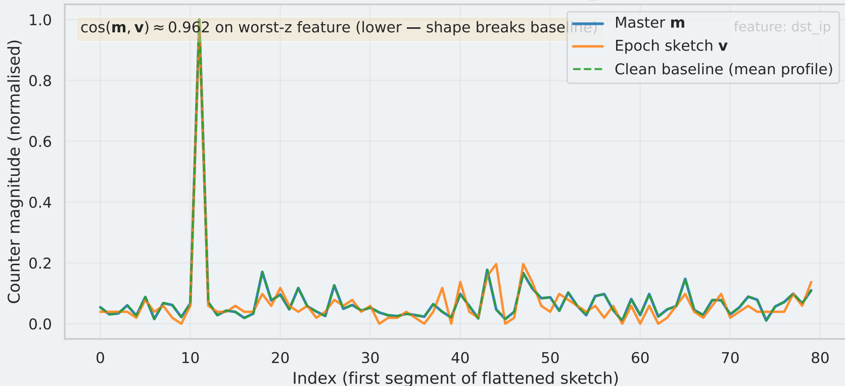
Attack epoch vs master (epoch 166 epoch_000166)
