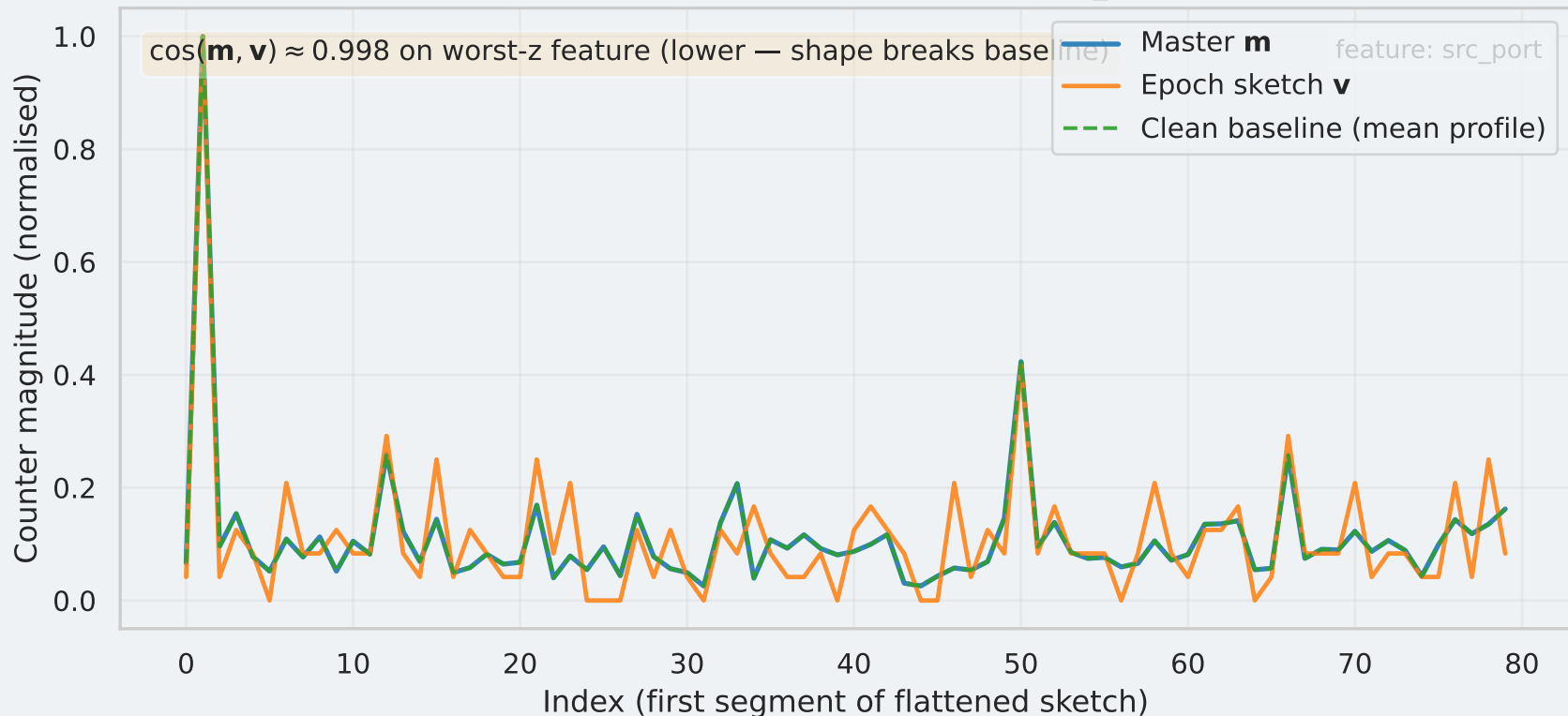
Attack epoch vs master (epoch 132 epoch_000132)
