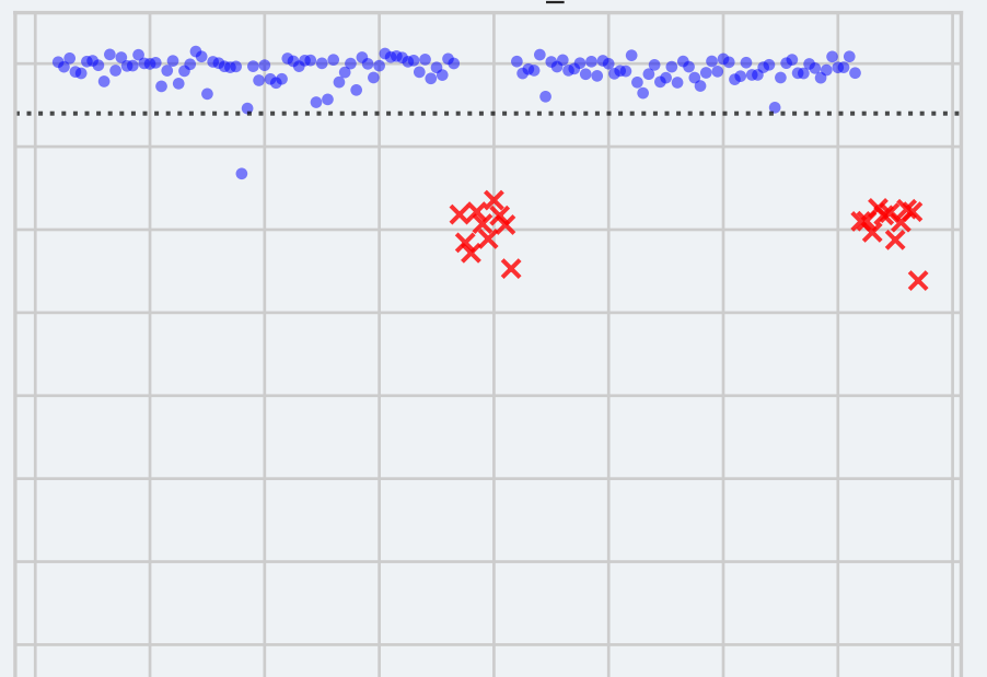
Feature: DST_PORT
