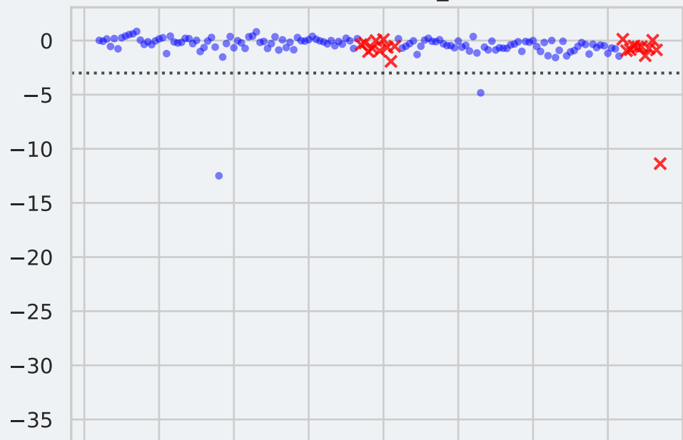
Feature: SRC_PORT
