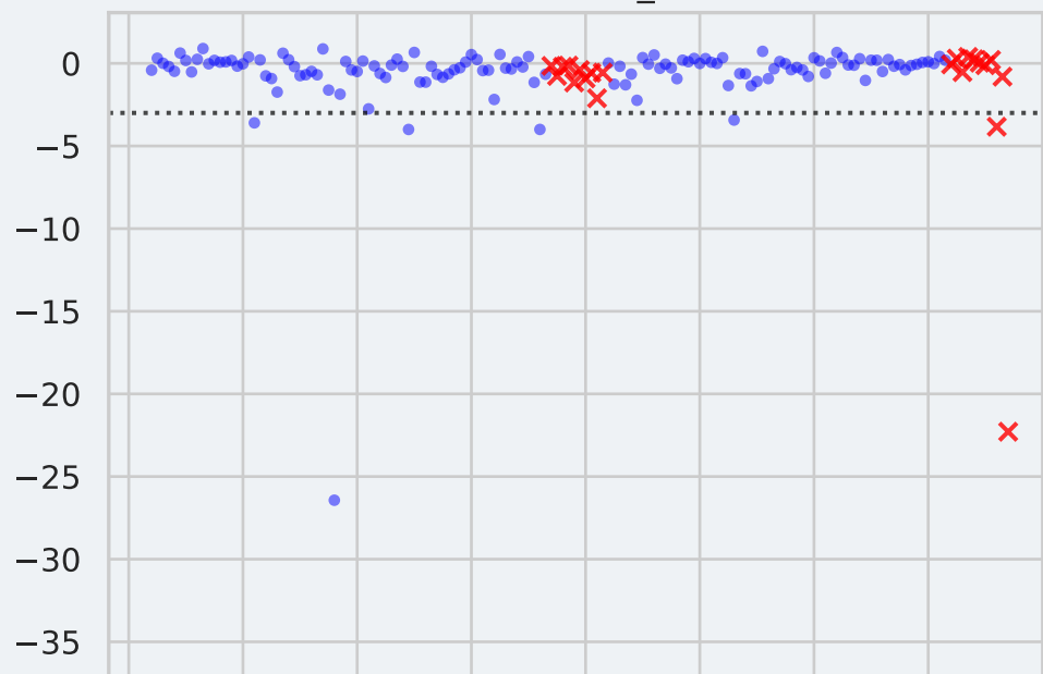
Feature: SRC_PORT
