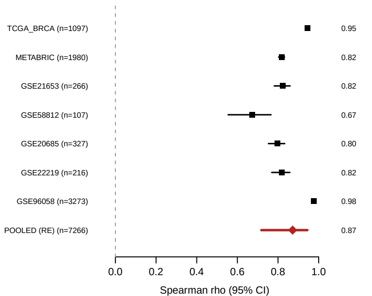
COL1A1~COL3A1 [unadjusted]
