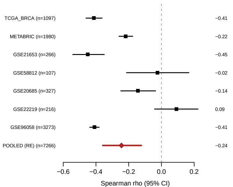
ETS1-&gt;COL1A1 [CAF-adjusted]
