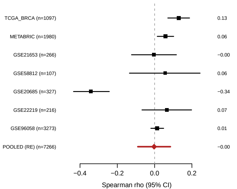
NFKB1-&gt;COL1A1 [unadjusted]
