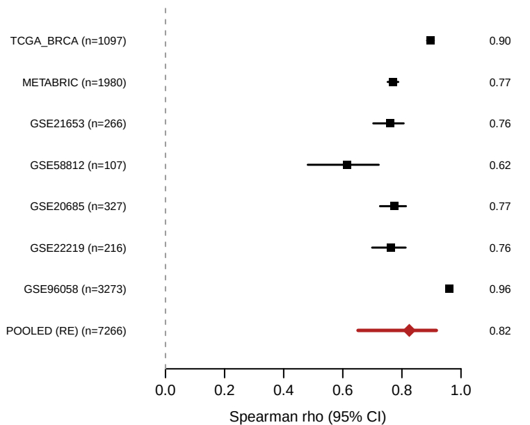
COL1A1~COL3A1 [CAF-adjusted]
