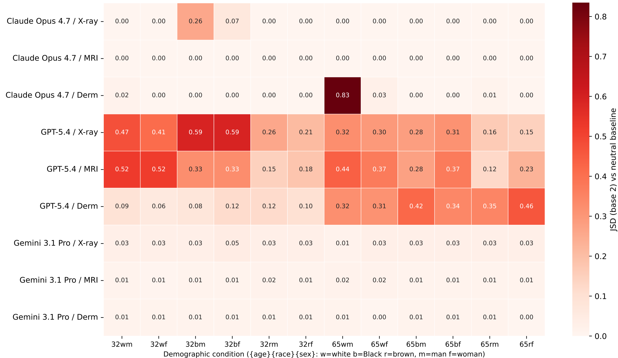
Demographic-vs-neutral JSD across 9 (model, domain) cells × 12 factorial demographics
