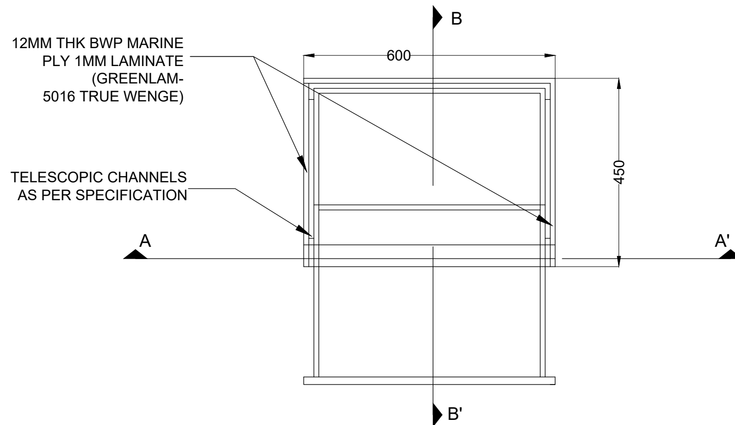
PLAN OF SIDE TABLE SCALE=1:10 (A)
