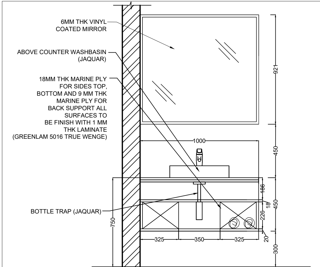
FRONT ELEVATION (A) SCALE= 1:20
