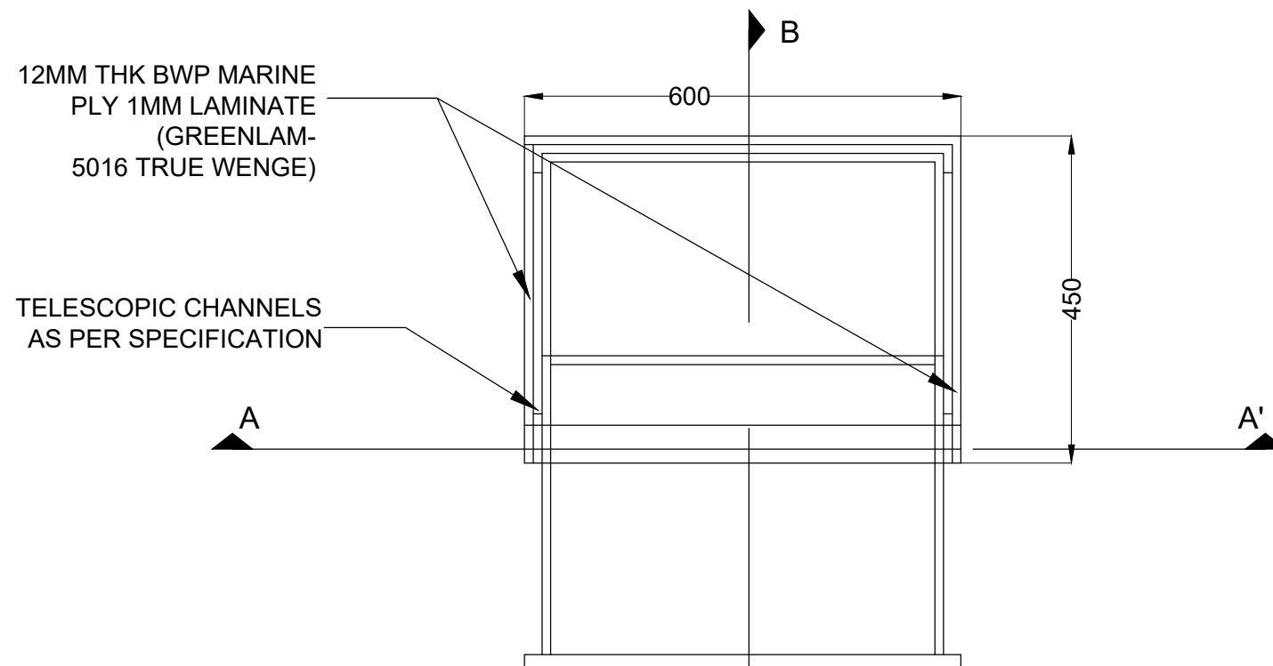
PLAN OF SIDE TABLE SCALE=1:10 (A)
