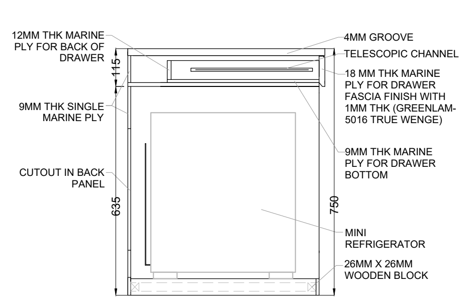
SECTION B-B' (C) SCALE= 1:75
