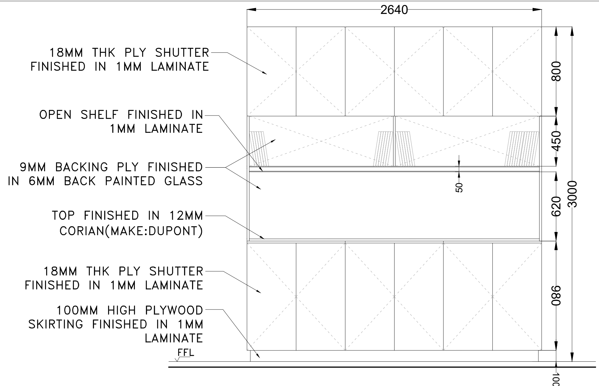
FRONT ELEVATION SCALE= 1:20 (C)
