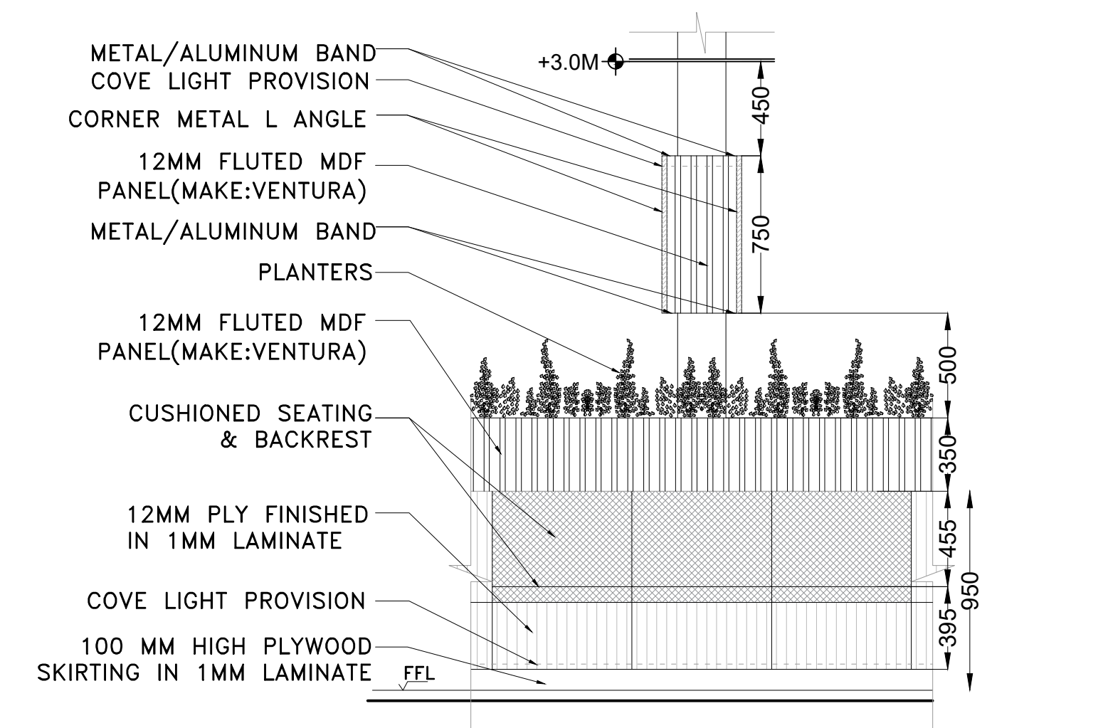
PART FRONT ELEVATION SCALE= 1:25
