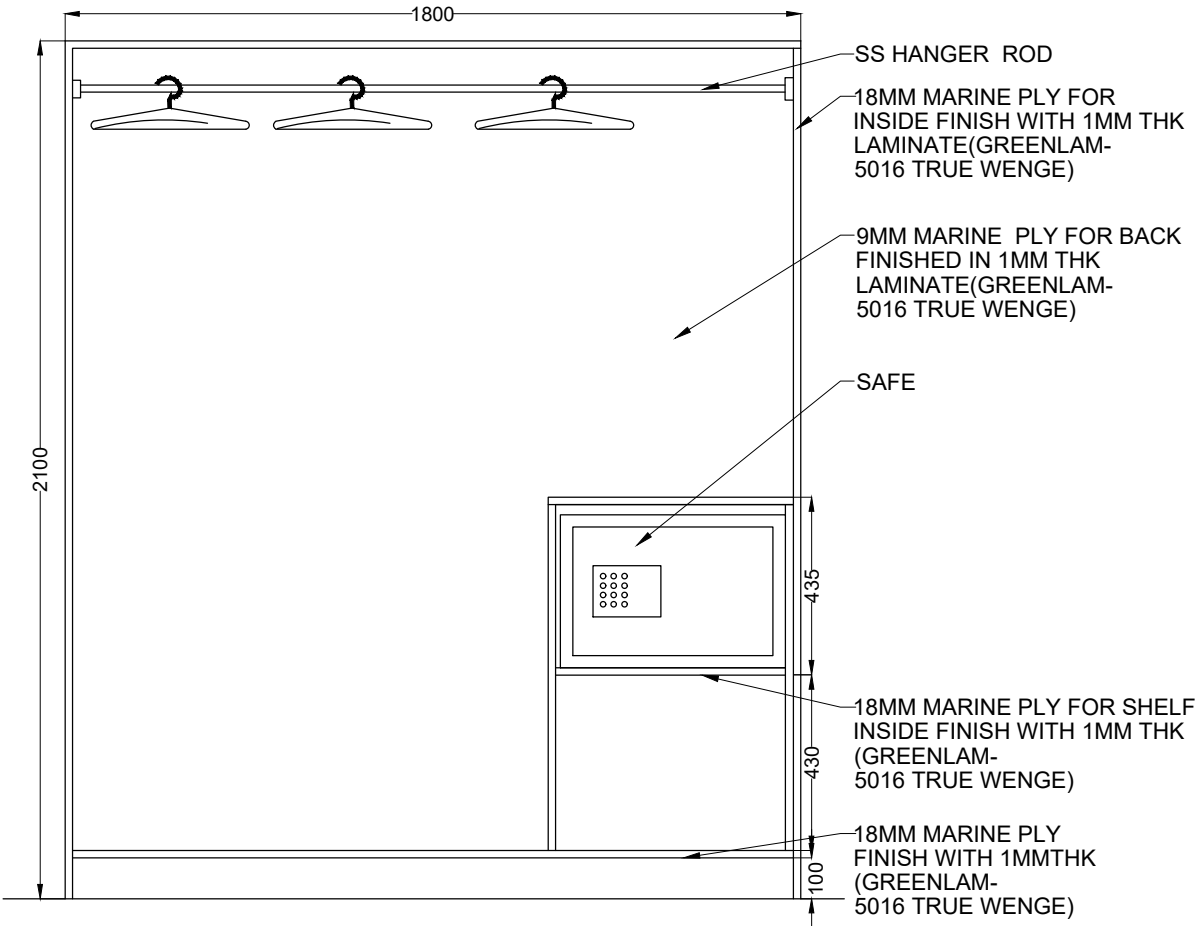
SECTION A-A' D SCALE=1:20
