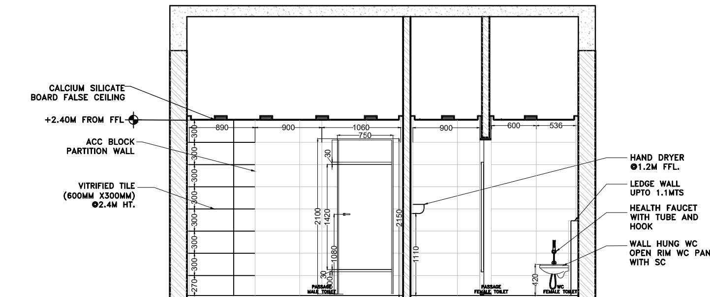
SECTION DD' SCALE= 1:50
