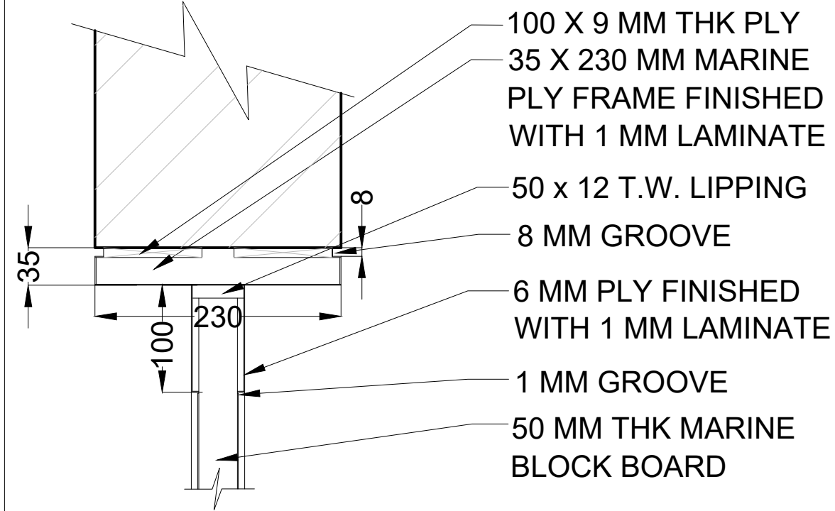
DETAIL AT A D SCALE= 1:5
