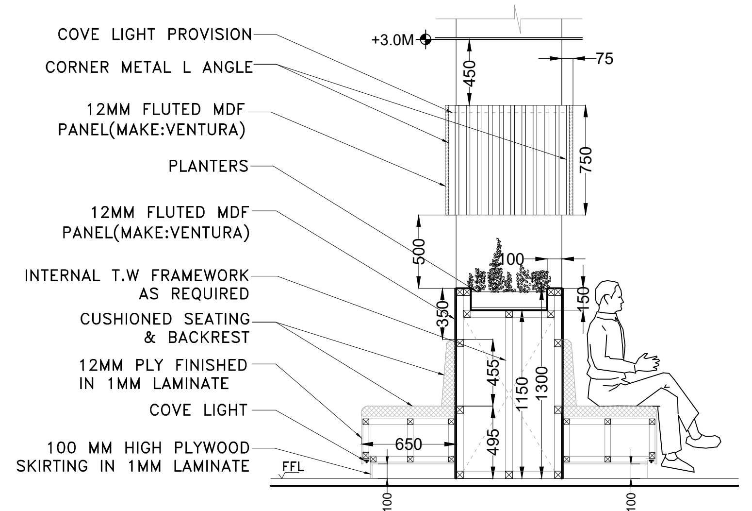
SECTION AA' C SCALE= 1:25
