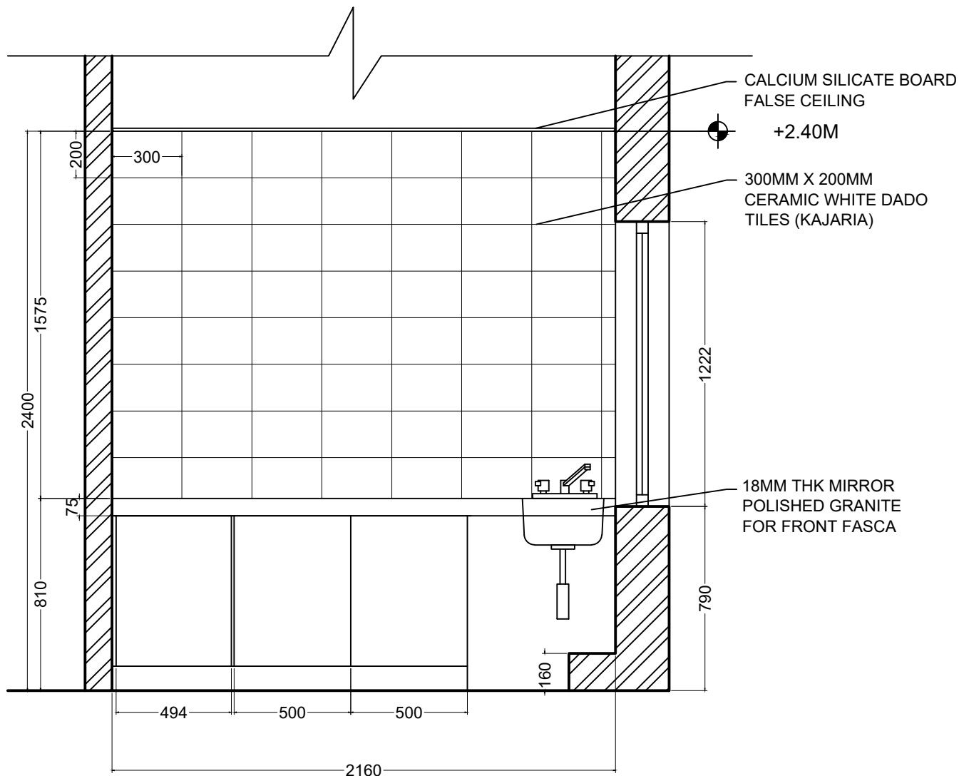
SECTION BB' SCALE=1:25 (C)
