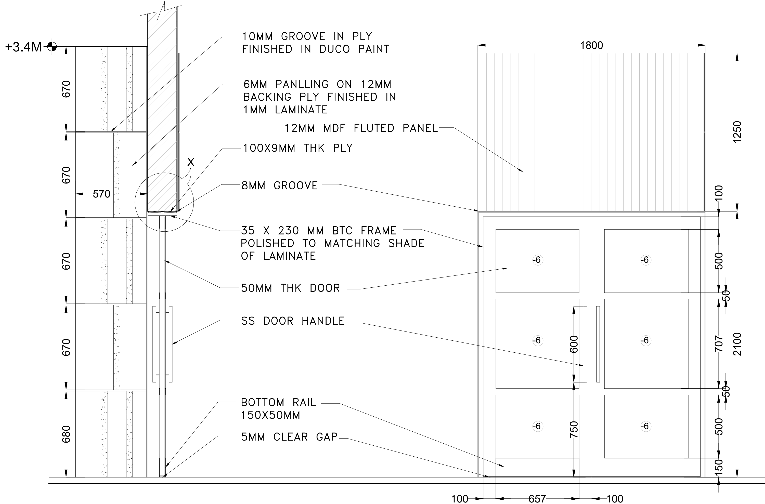
SECTION AA' B SCALE= 1:15
