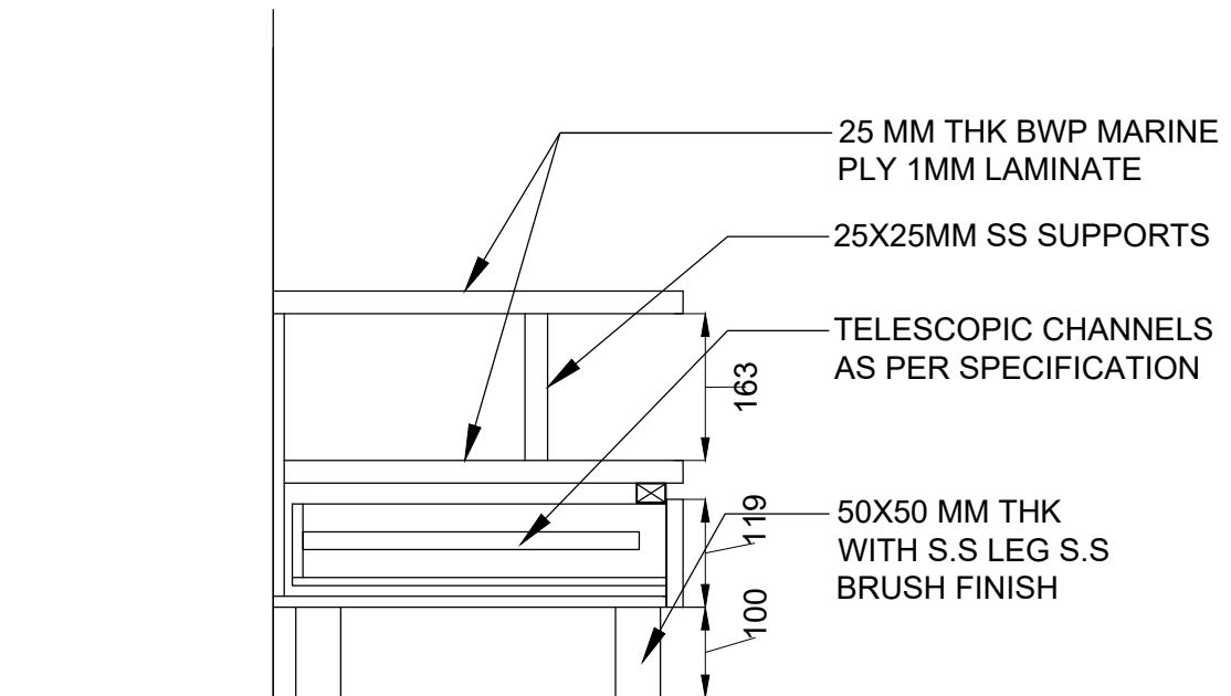
SECTION B-B' SCALE= 1:10 (C)
