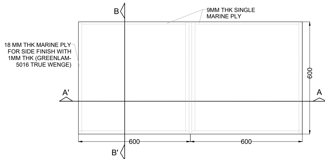
PLAN OF SIDE TABLE SCALE=1:10 Ⓐ
