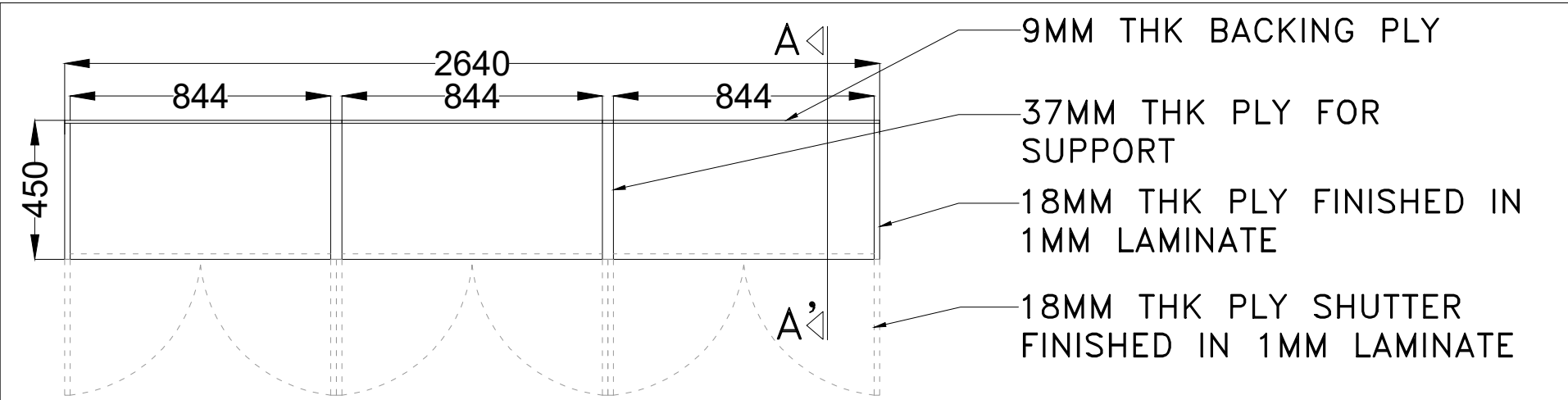
STORAGE UNIT PLAN AT 0.75M SCALE= 1:20 (A)
