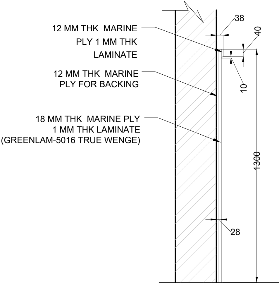
SECTION A-A' (B) SCALE= 1:20
