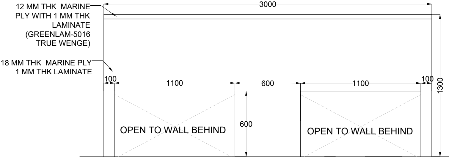
FRONT ELEVATION (C) SCALE= 1:25
