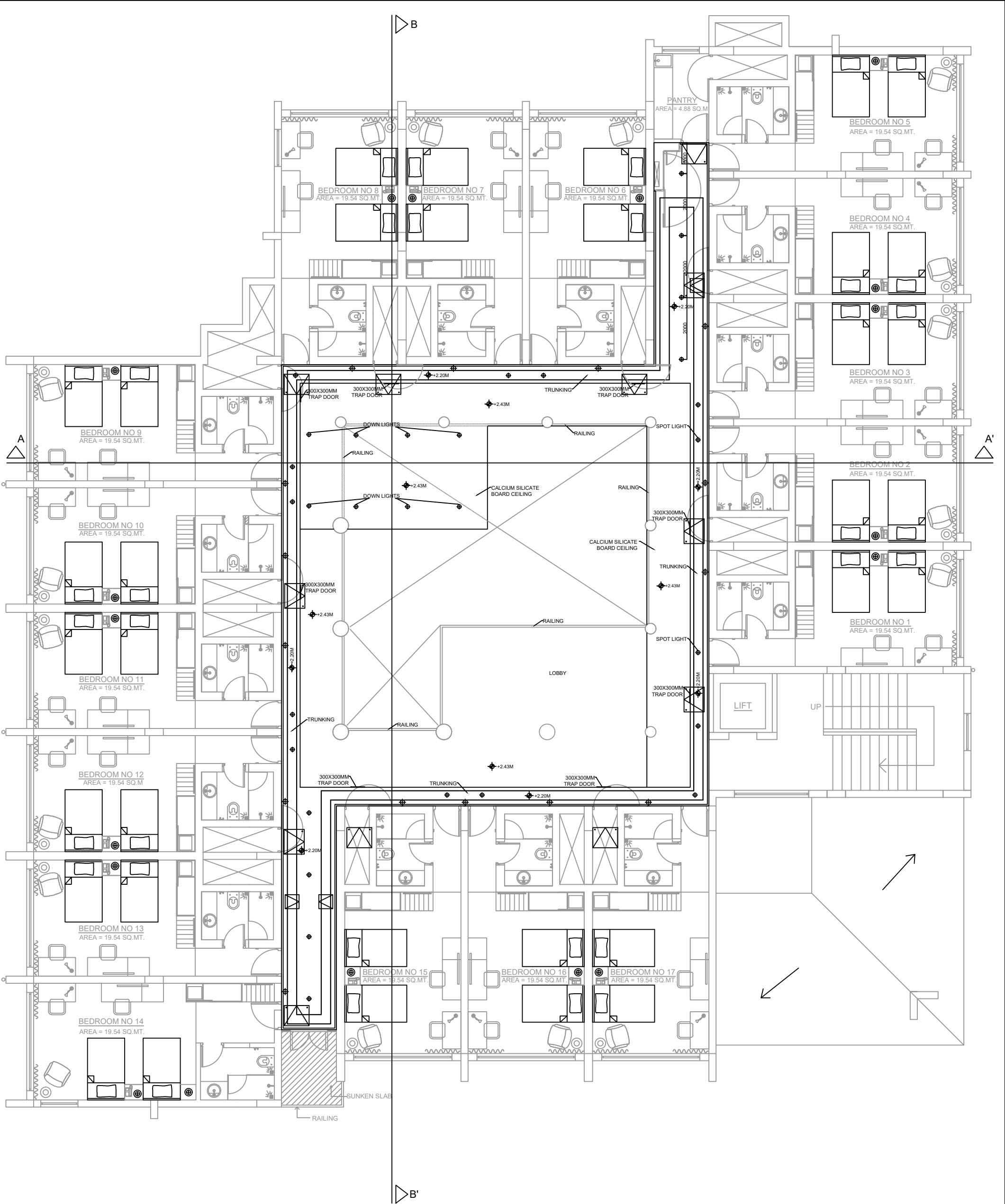
FIRST FLOOR PLAN SCALE=1:500
