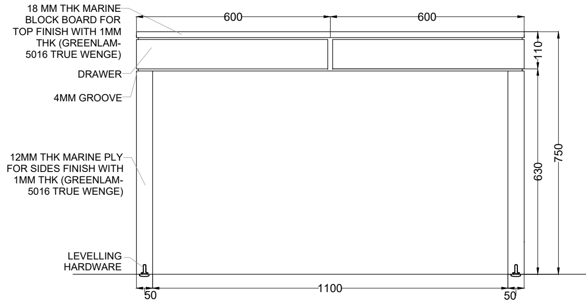
FRONT ELEVATION SCALE=1:10 ⓑ
