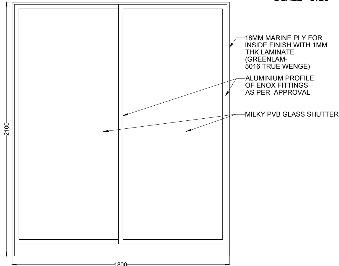
FRONT ELEVATION B SCALE=1:20
