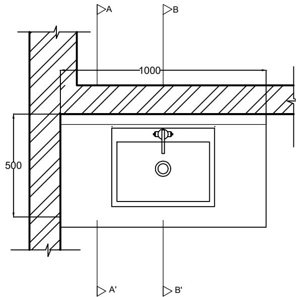
PLAN OF WASHBASIN COUNTER (C) SCALE= 1:20
