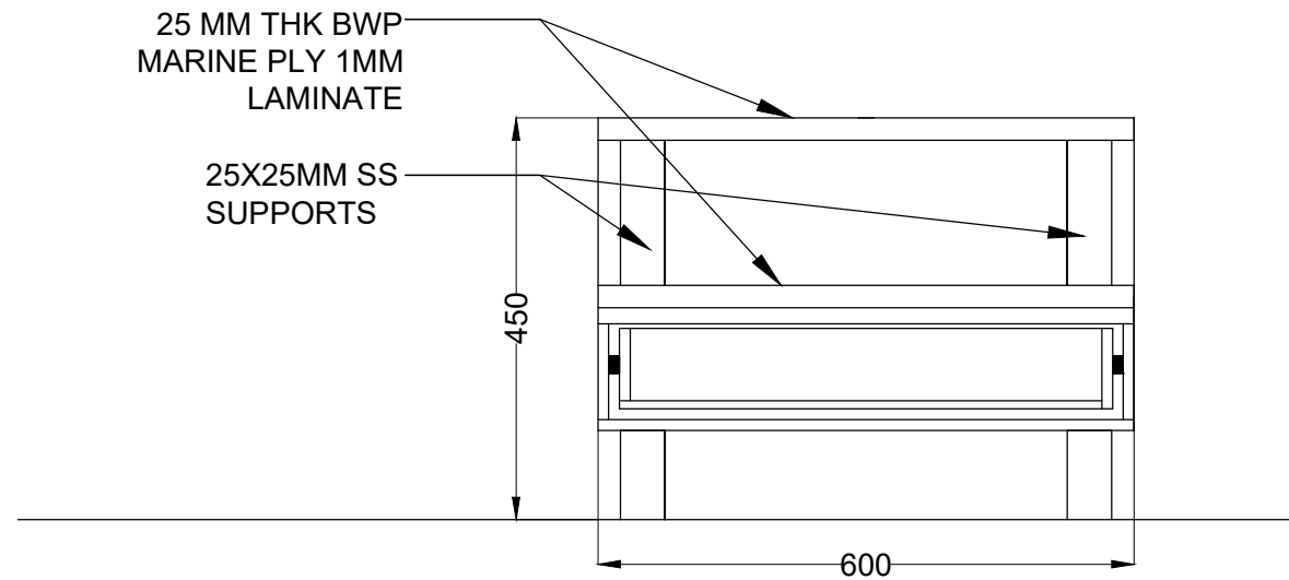
SECTION A-A' SCALE= 1:10 (B)
