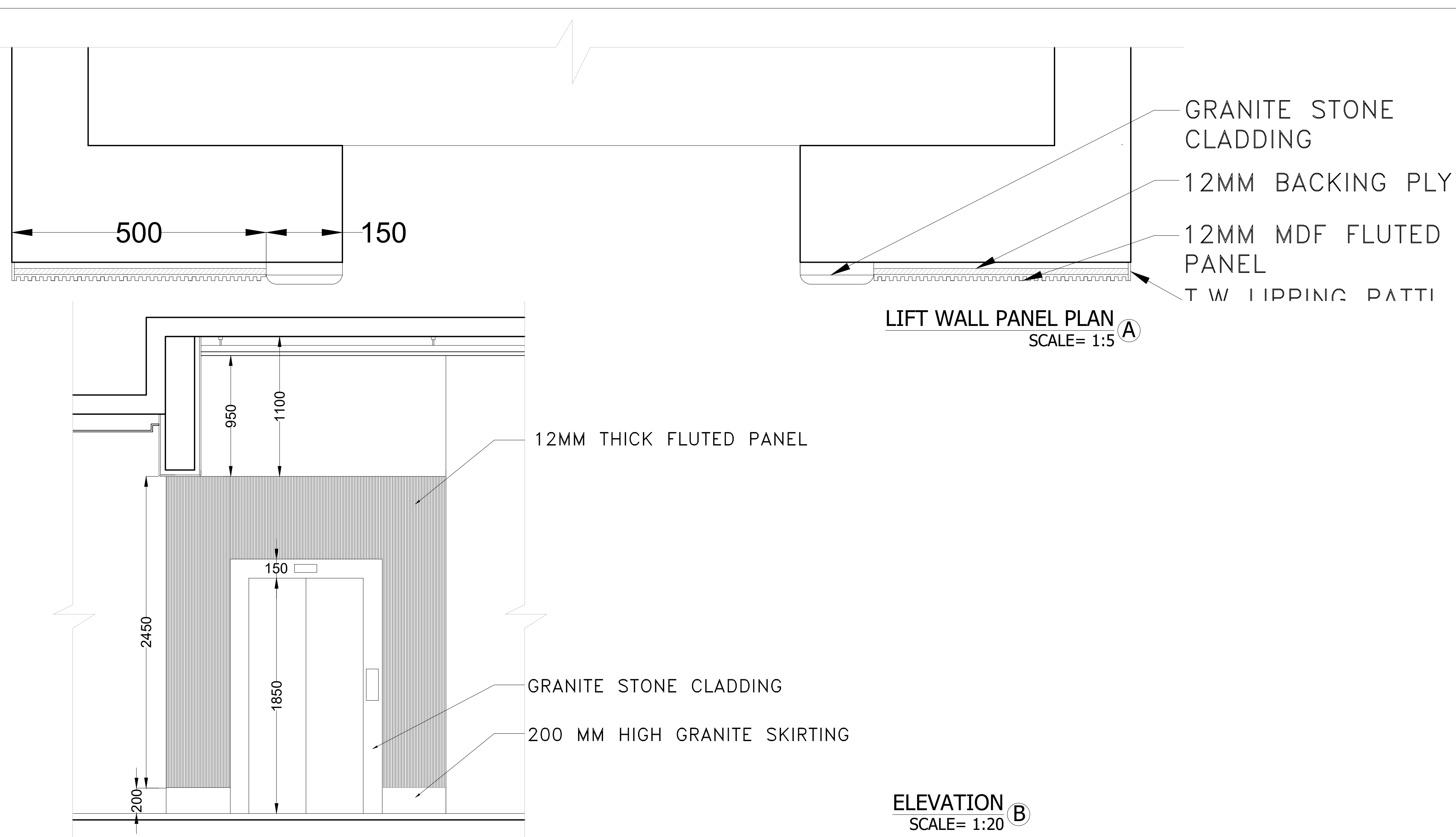
LIFT WALL PANEL DETAIL-08
