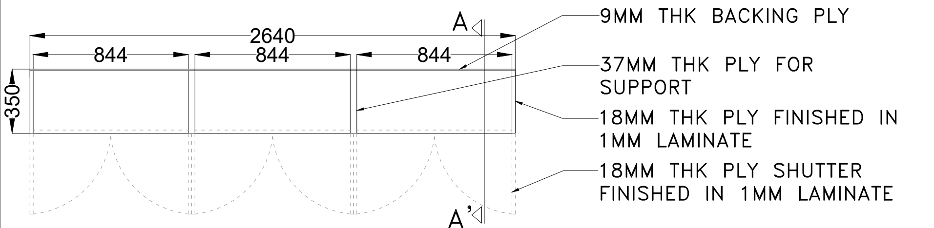
STORAGE UNIT PLAN AT 2.2M SCALE= 1:20 (B)
