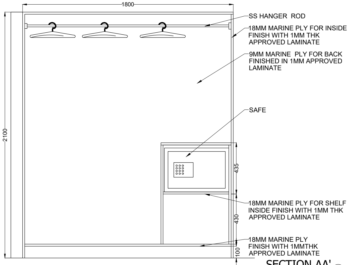
SECTION AA' D SCALE= 1:20
