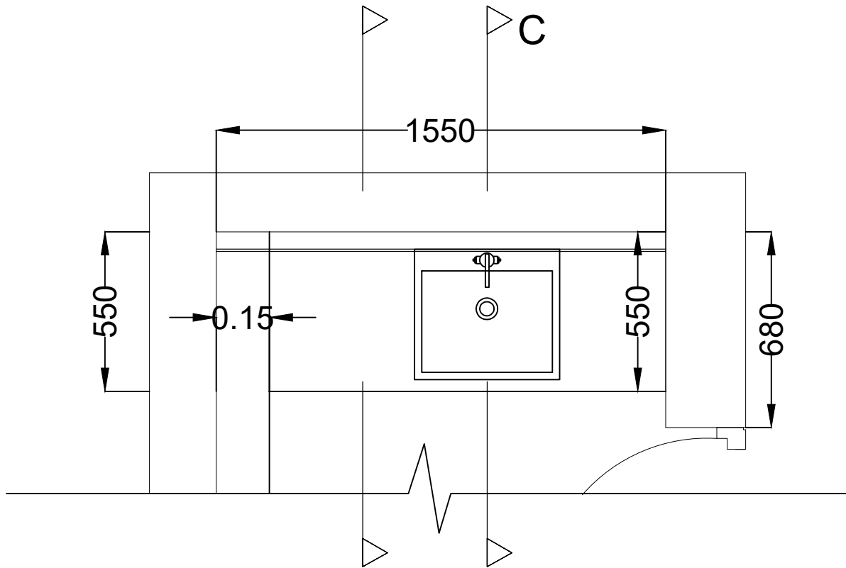
PLAN OF WASH BASIN COUNTER SCALE=1:20
