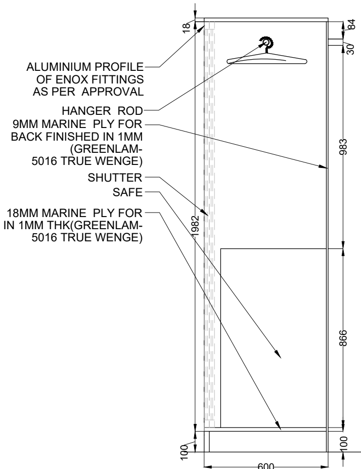
SECTION B-B' C SCALE=1:20
