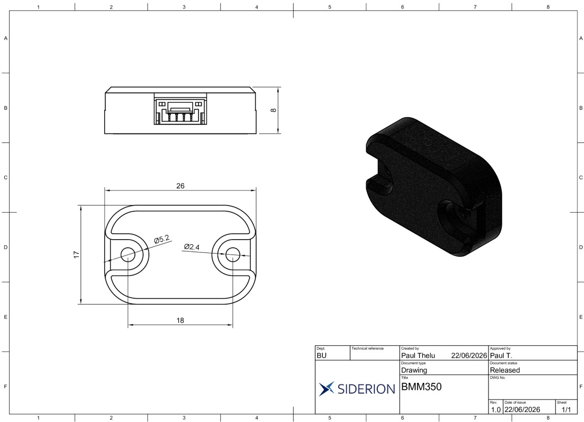
Figure 5. BMM350 v1.0 mechanical drawings
