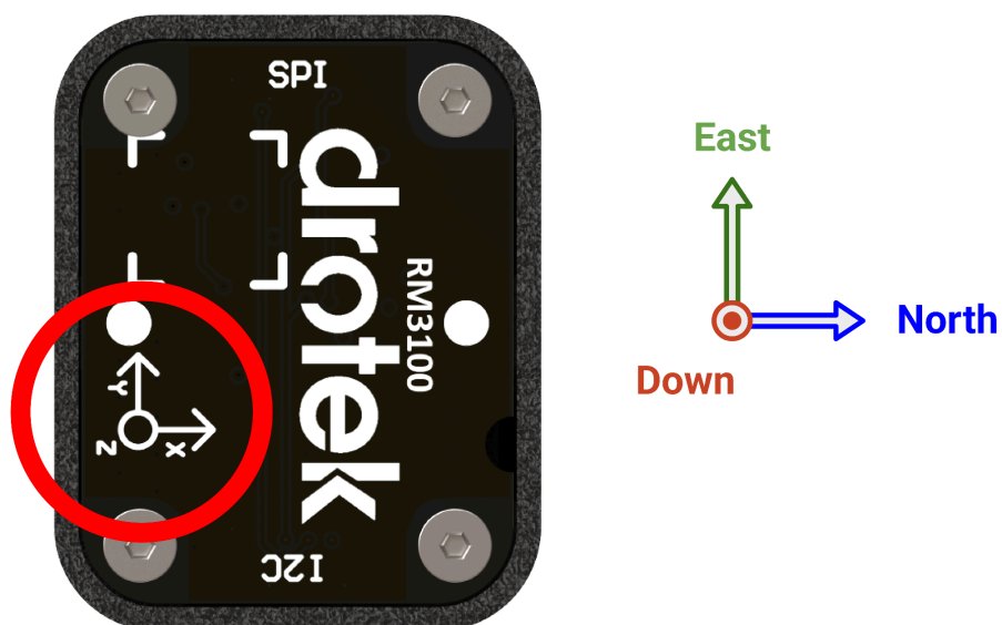
Figure 1. RM3100 - NED (XYZ) orientation (bottom view)
