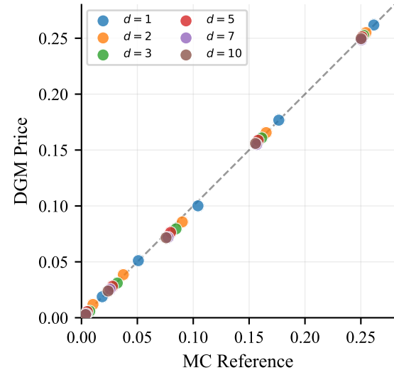
DGM vs MC
