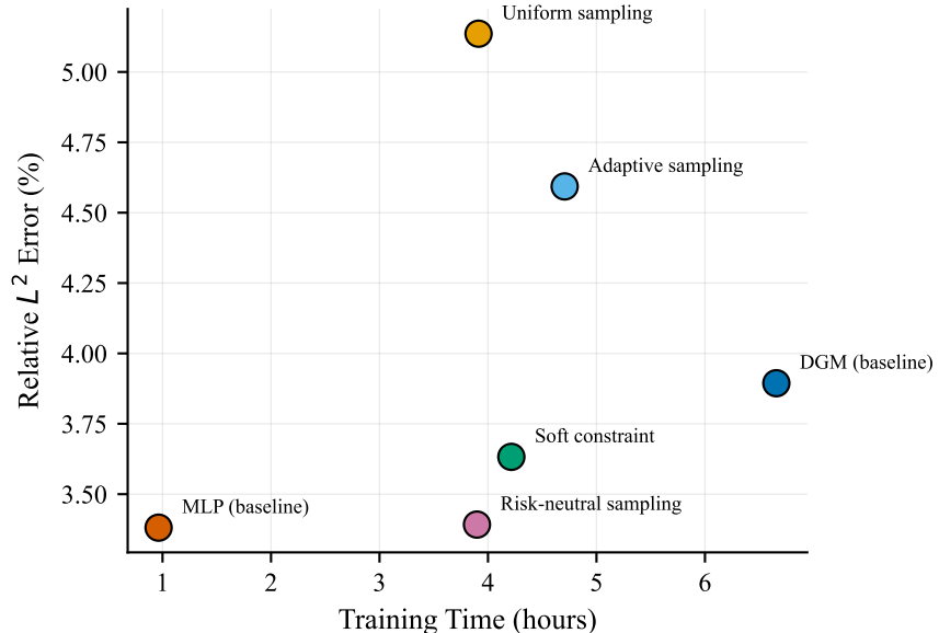
Accuracy vs. Computational Cost
