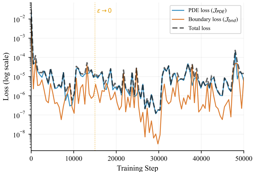
Component-wise Loss Decomposition ( d = 2 , DGM)
