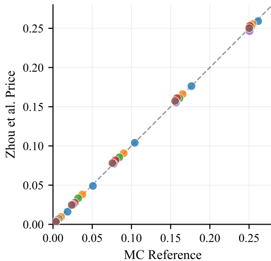
Zhou et al. vs MC
