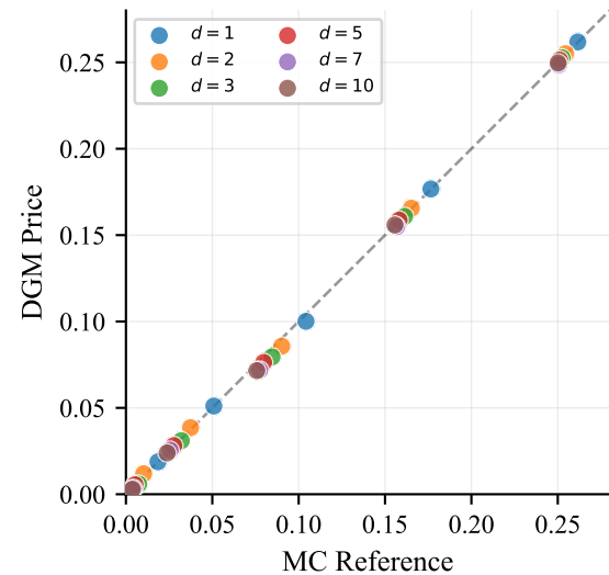
DGM vs MC
