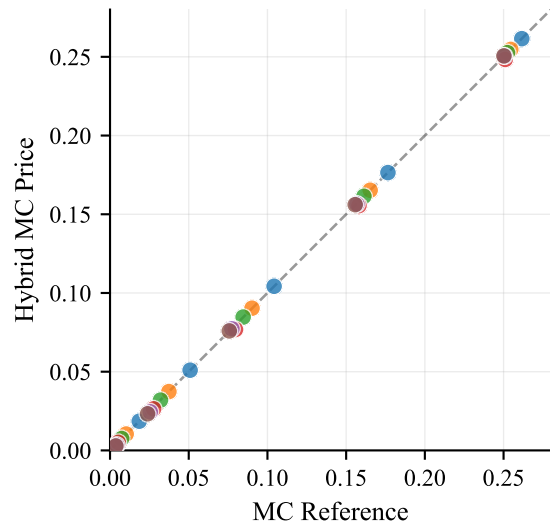
Hybrid MC vs MC
