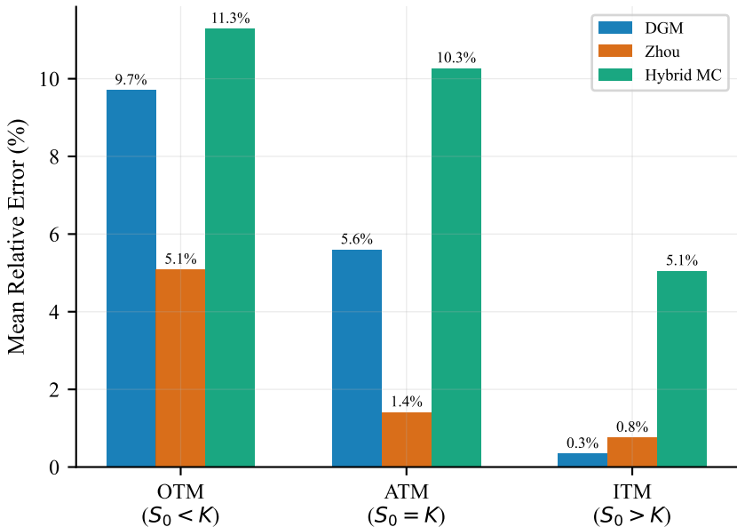
Pricing Error by Moneyness Region
