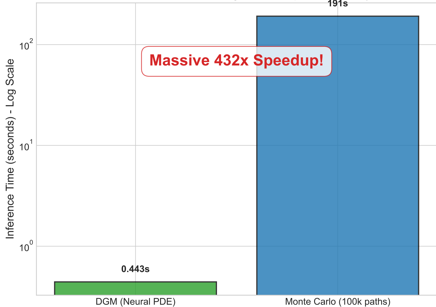
Time-to-Solution: Pricing 10,000 Options ( d = 5 )
