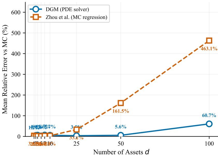
Pricing Error vs. Problem Dimension
