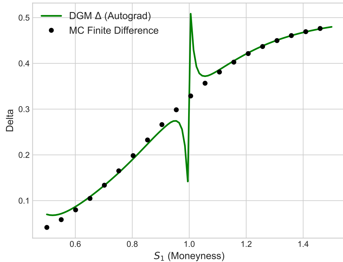
\Delta = \partial V / \partial S_1
