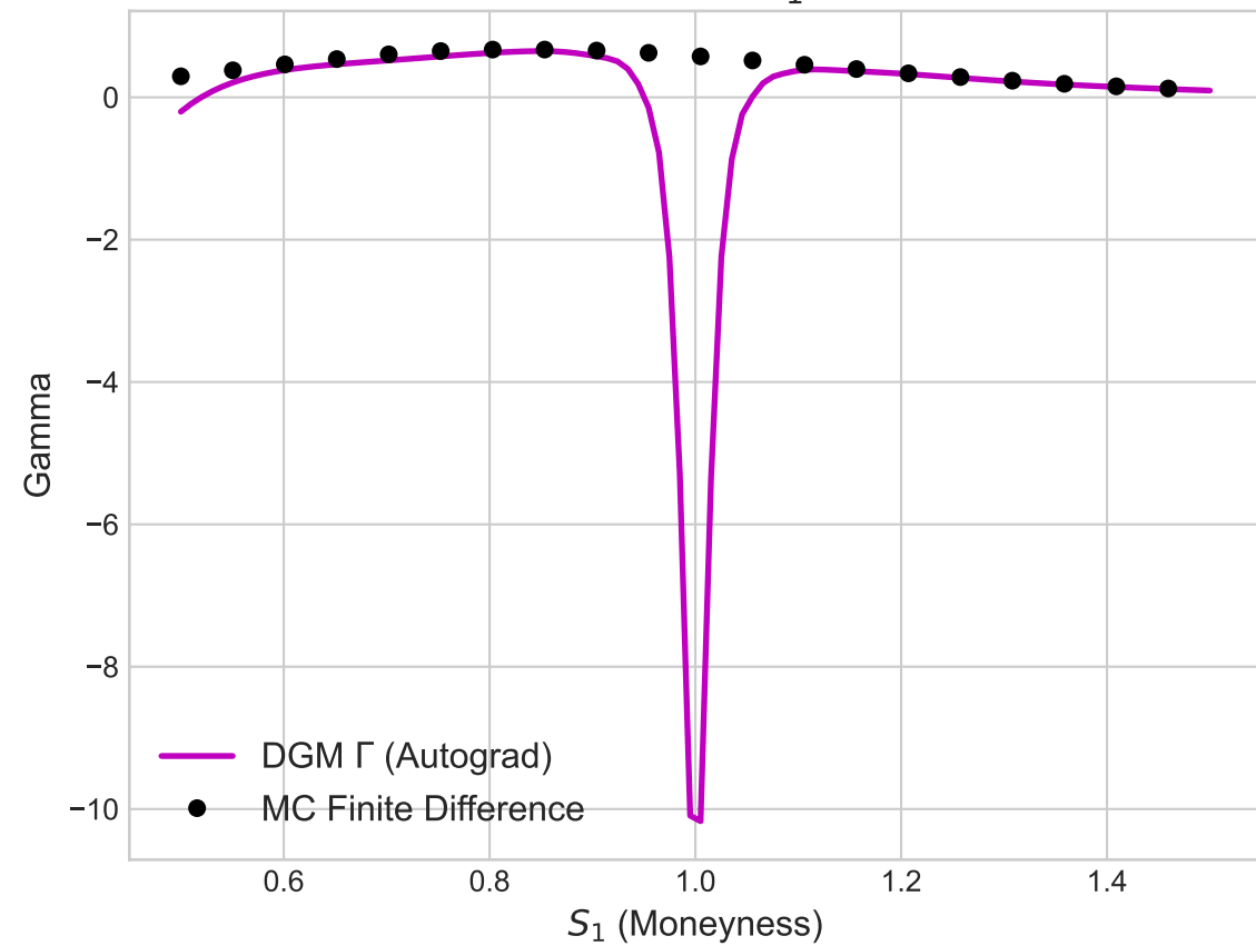
\Gamma = \partial^2 V / \partial S_1^2
