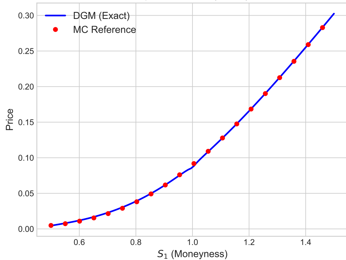
Option Price V ( d = 2 )
