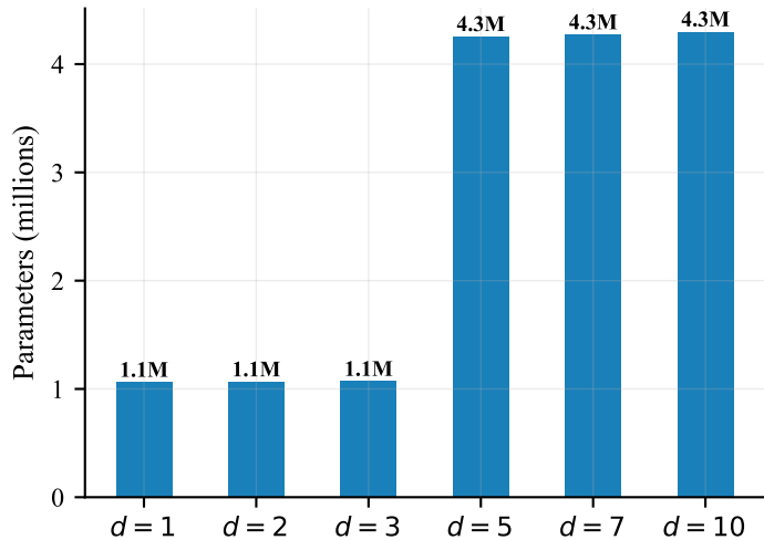
Model Size vs. Dimension
