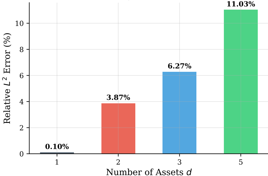
DGM Pricing Error vs Dimension
