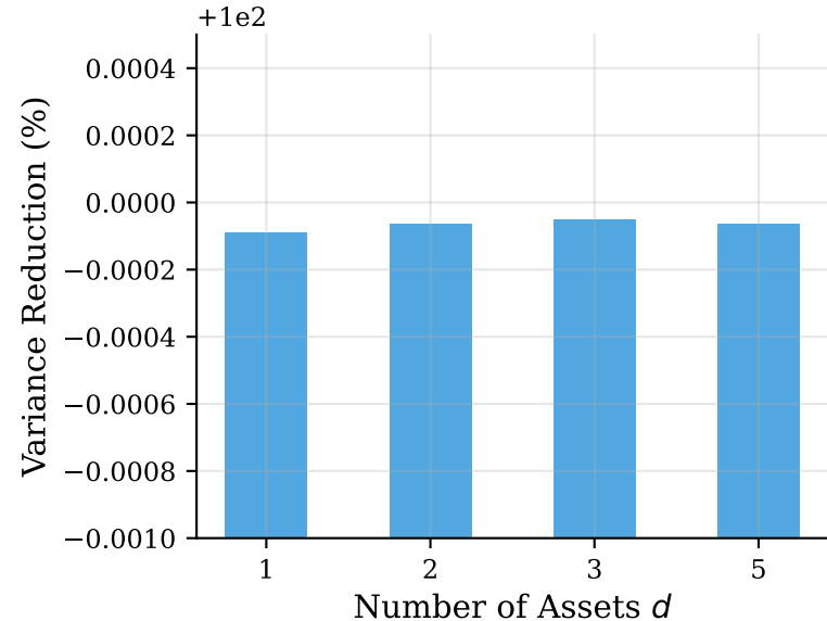
Hybrid DGM-MC: Variance Reduction
