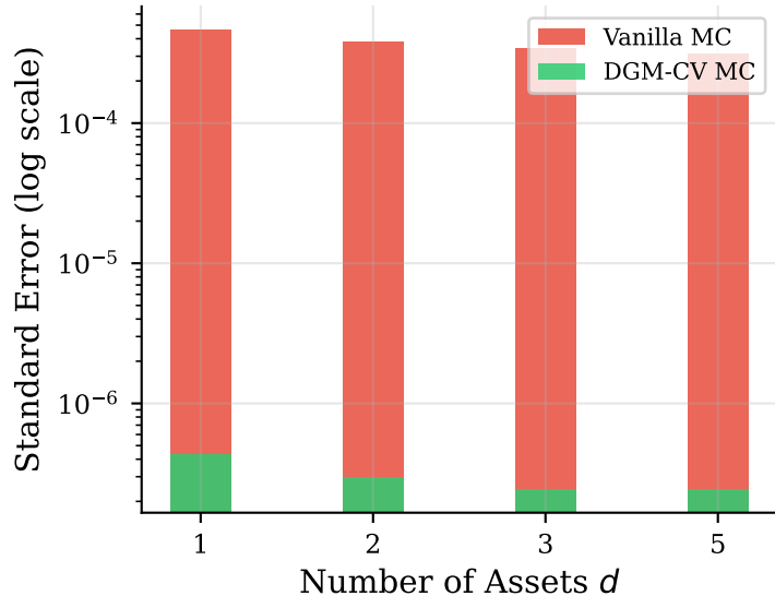
Standard Error Comparison
