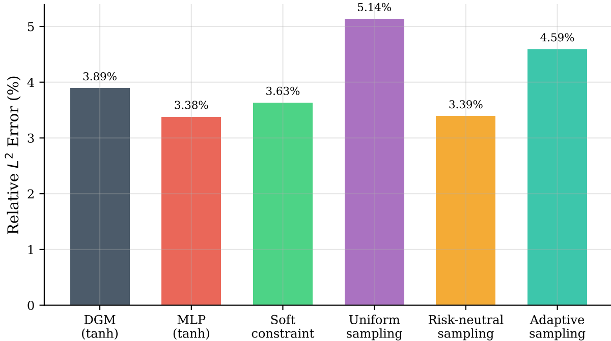
Ablation Study ( d = 2 , Basket Call, 50k steps)
