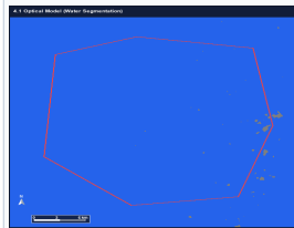
RS-VLM + Segmentation
