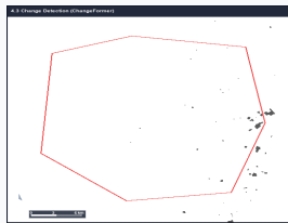
Pixel ChangeFormer
