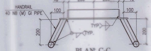
PLAN C-C (SCALE 1:10)
