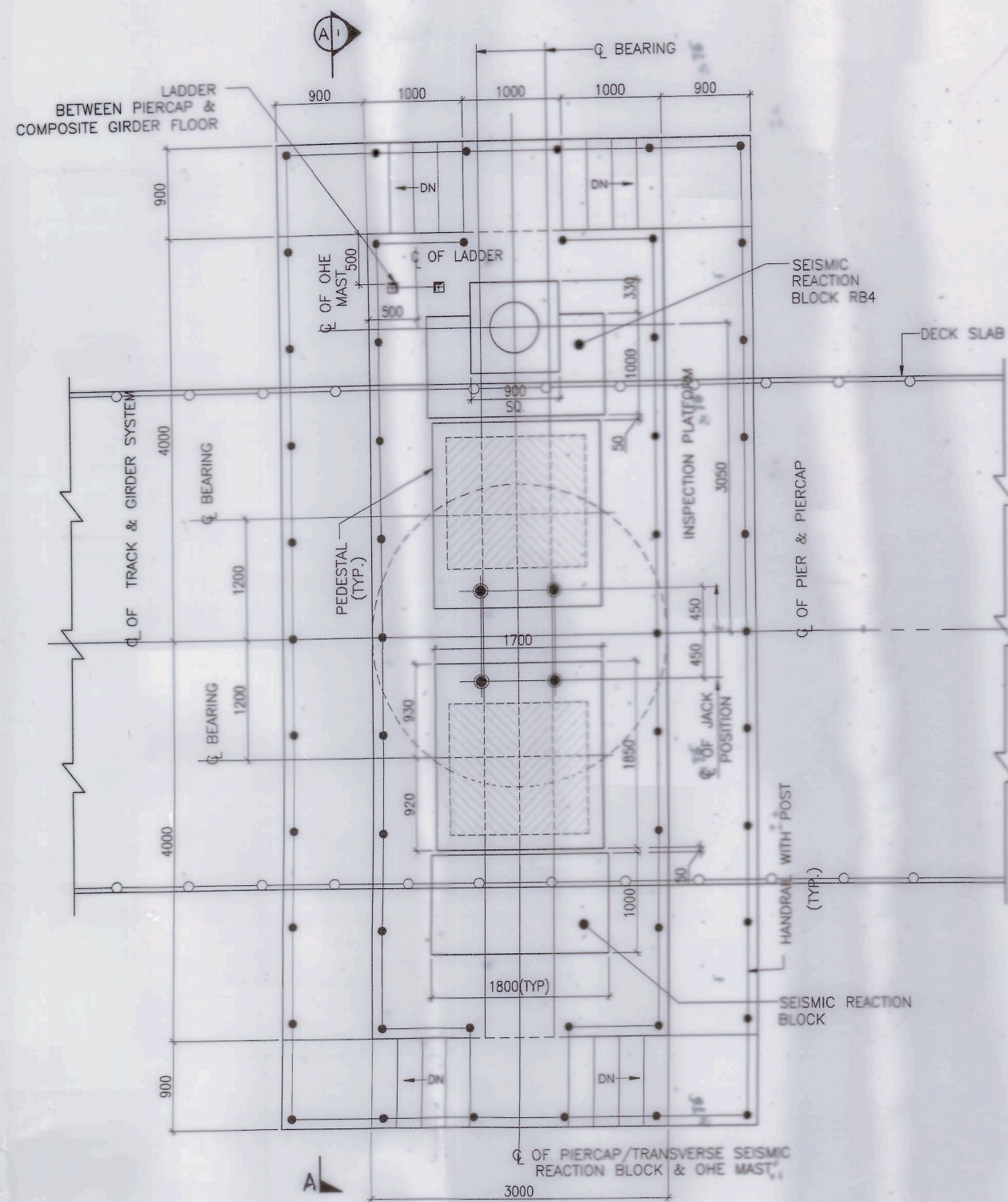
PLAN OF PIERCAP (SCALE 1:40)
