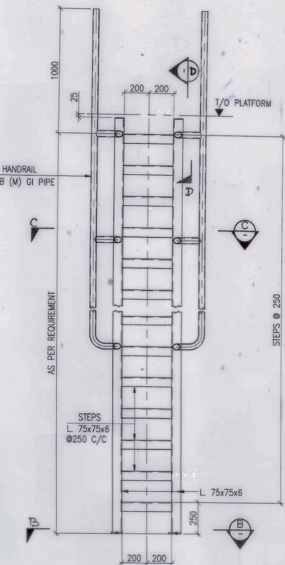
TYPICAL DETAIL OF LADDER (SCALE 1:20)
