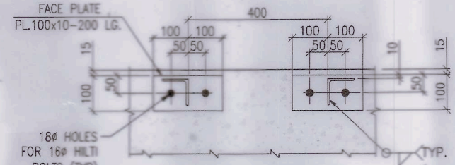
PLAN E-E (SCALE 1:10)
