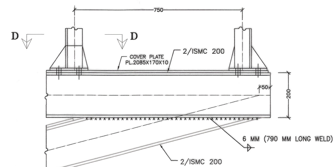
DETAILS AT '3' & '4' (SCALE-1:10)
