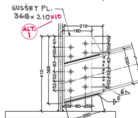
DETAILS AT '2' (SCALE-1:10)
