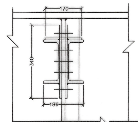
VIEW AT C-C (SCALE-1:10)
