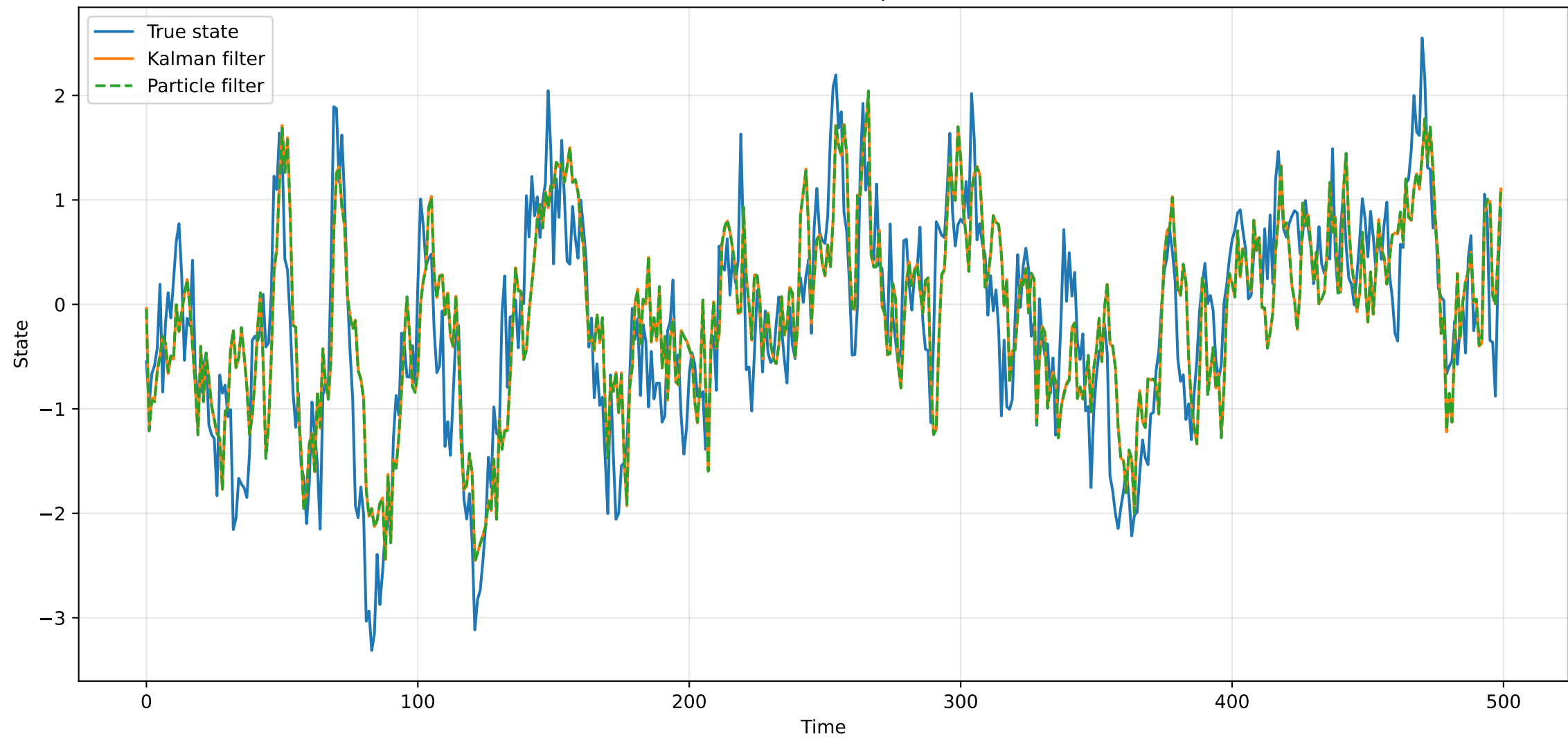
Kalman Filter vs Bootstrap Particle Filter
