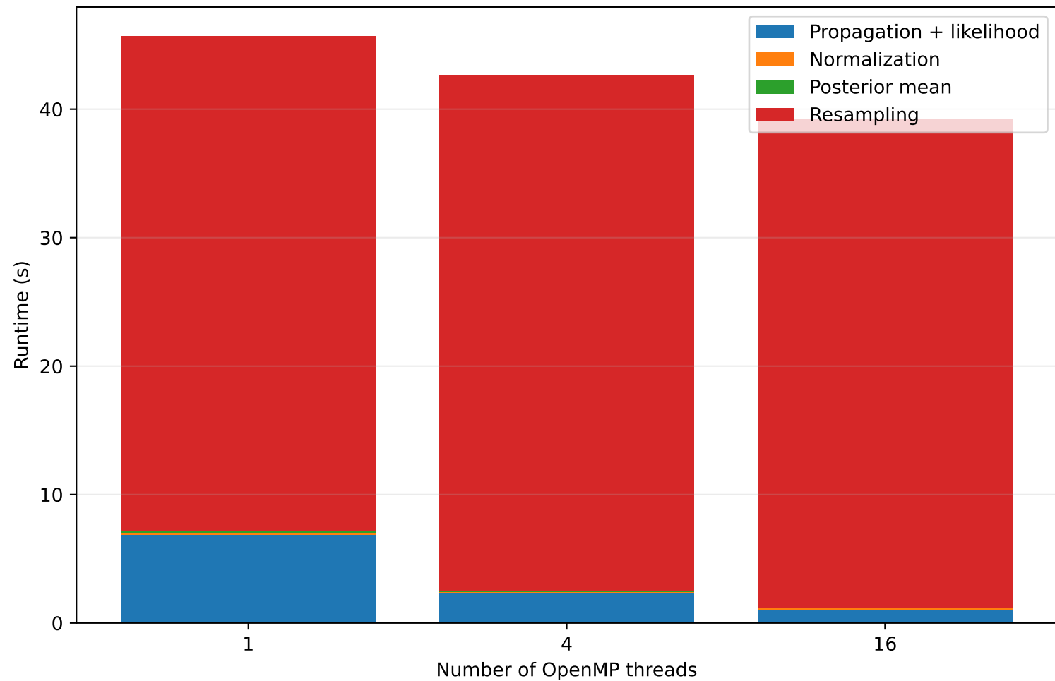
Runtime decomposition for N = 500,000
