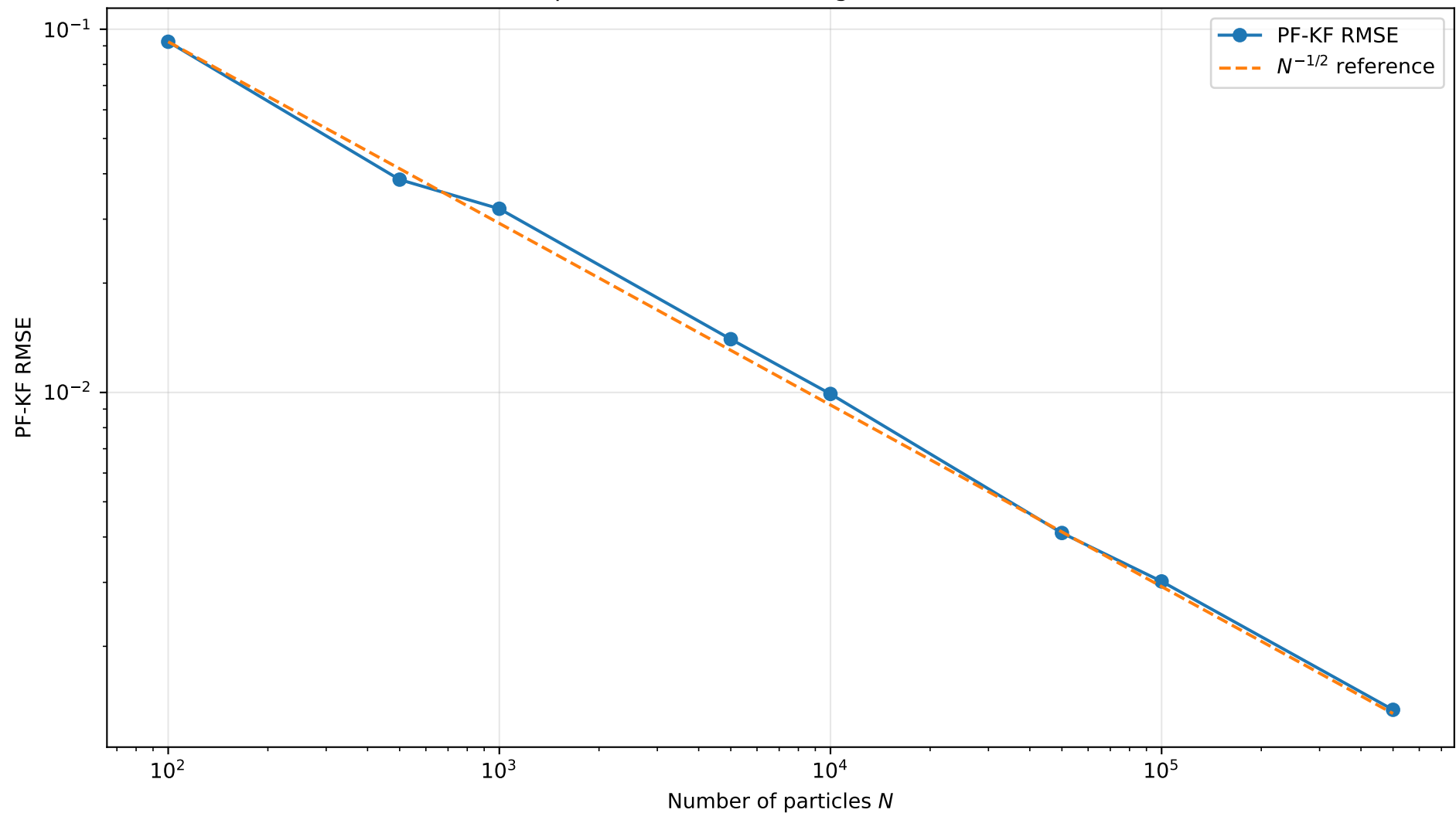
Bootstrap Particle Filter Convergence to Kalman Filter
