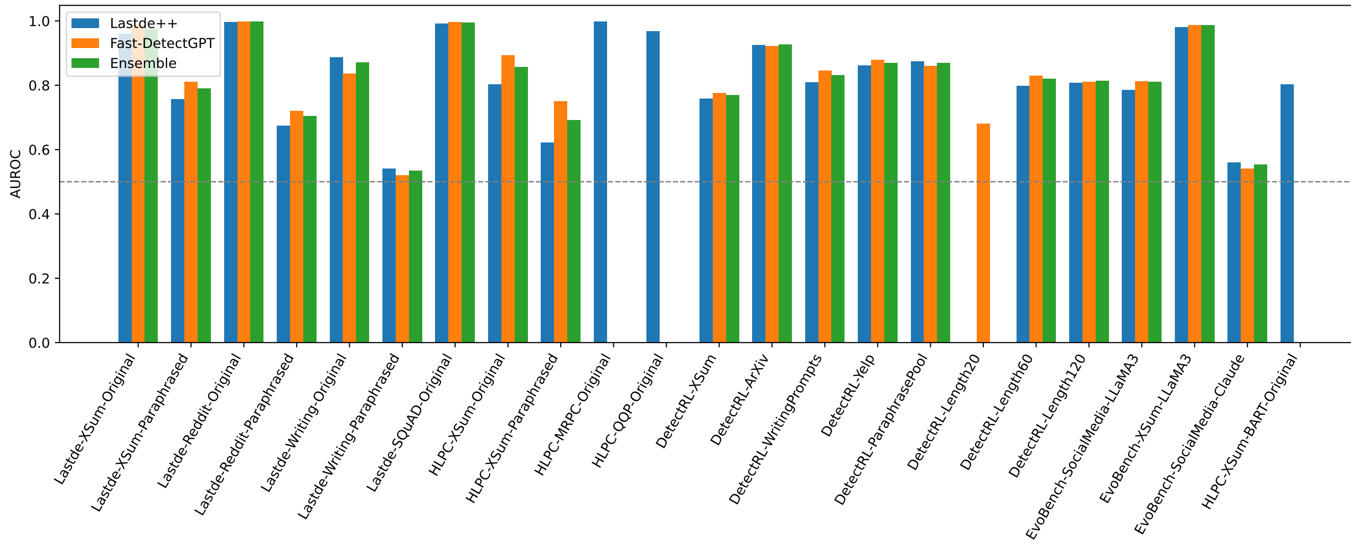
AUROC Across All Tested Conditions
