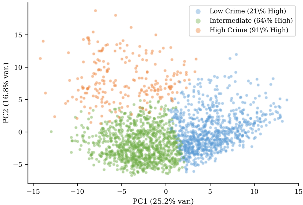
K-Means Clusters ( K = 3 ) in PC Space
