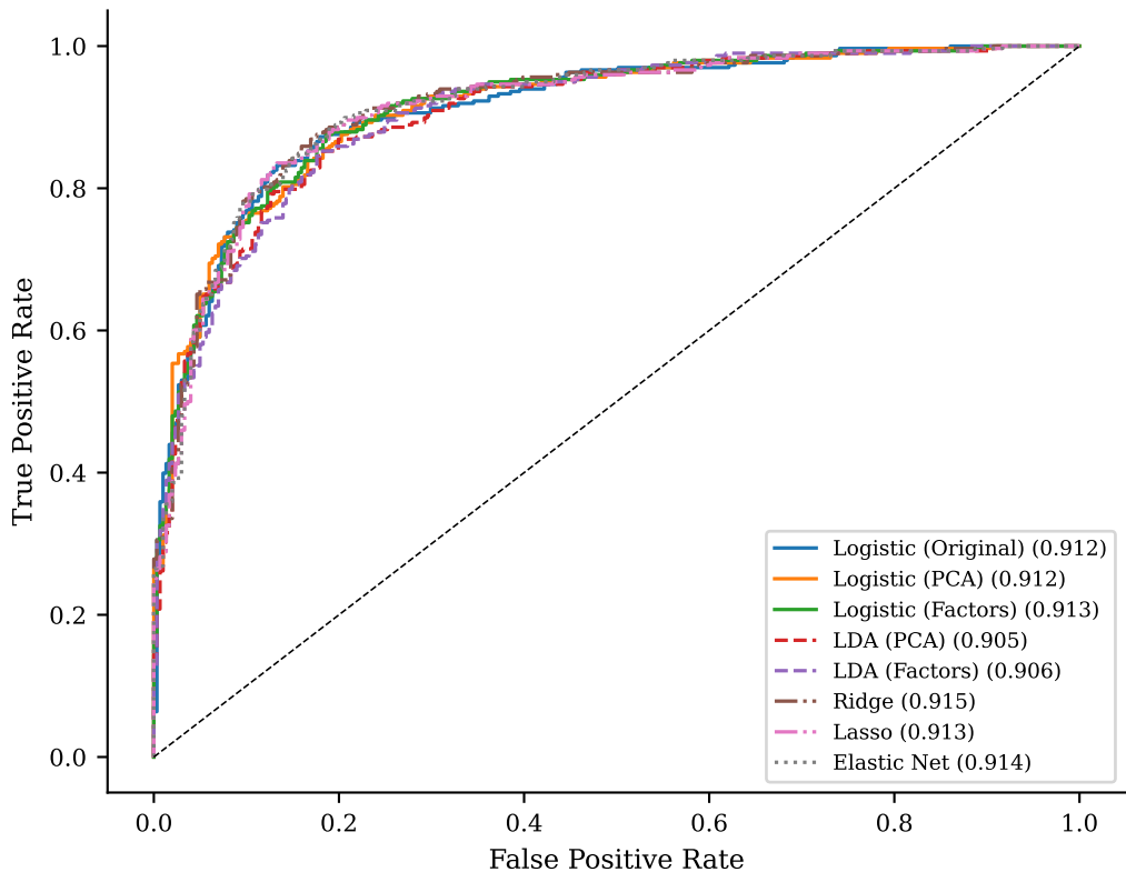
ROC Curves — All Classification Models
