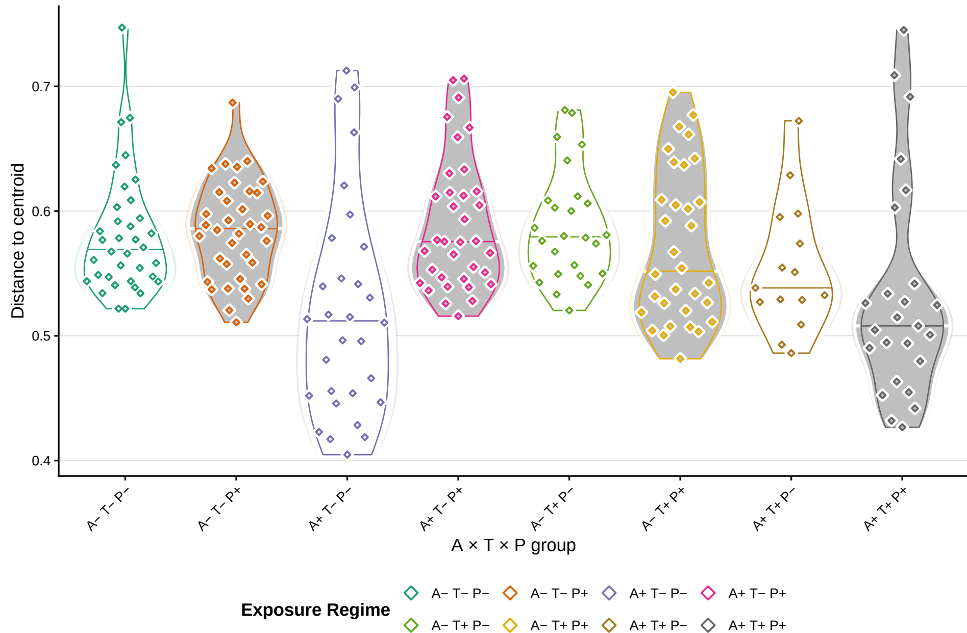
Beta diversity dispersion by factorial exposure regimes (Canberra)
