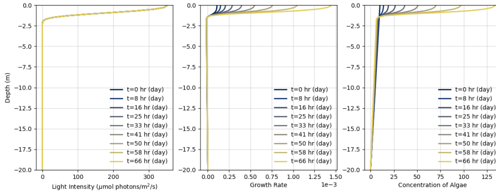
Figure 4: Algae Concentration with constant light
