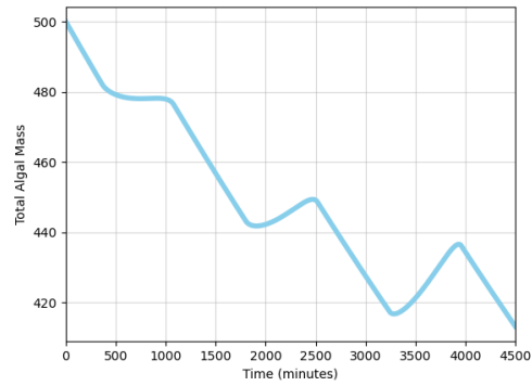
Figure 6: Total algal mass with diurnal light over time.
