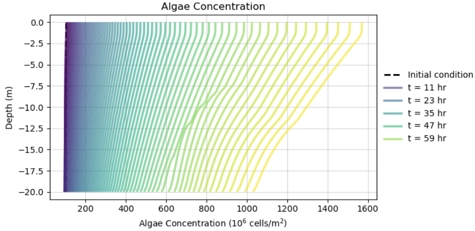
Figure 9: Algae Concentration with constant light + flow
