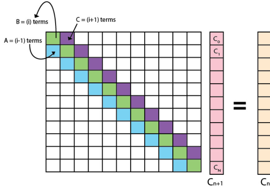
Figure 3: Tridiagonal matrix for implicit scheme
