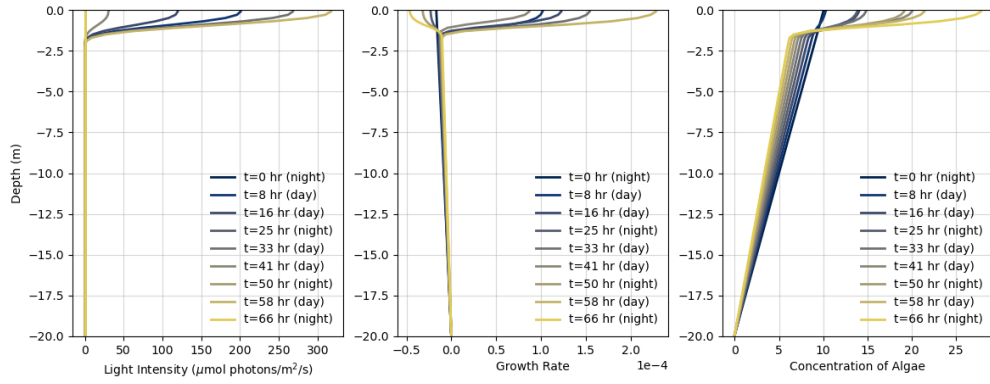
Figure 5: Algae Concentration with diurnal light
