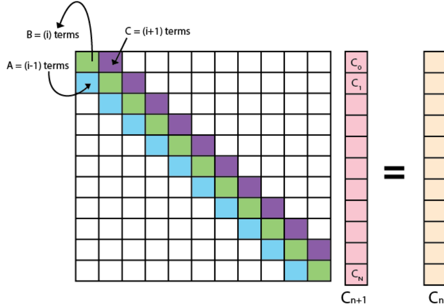
Figure 2: Tridiagonal matrix for implicit scheme
