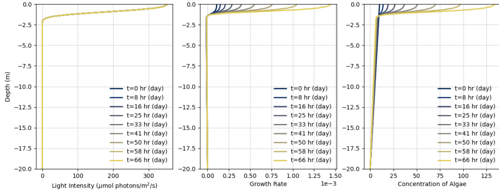
Figure 3: Algae Concentration with constant light
