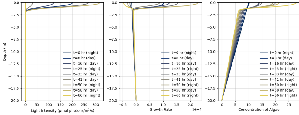
Figure 4: Algae Concentration with diurnal light
