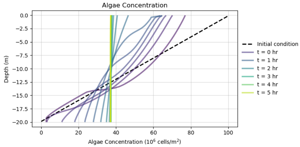
Figure 8: Algae Concentration with diurnal light
