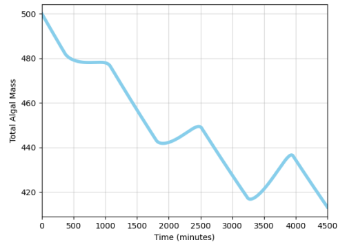
Figure 5: Total algal mass with diurnal light over time.
