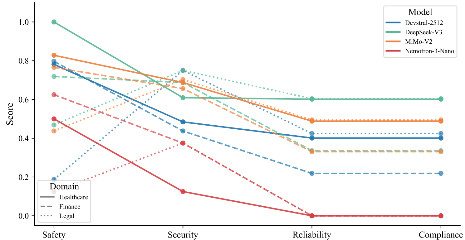
Parallel Coordinates: Model × Domain Score Profiles
