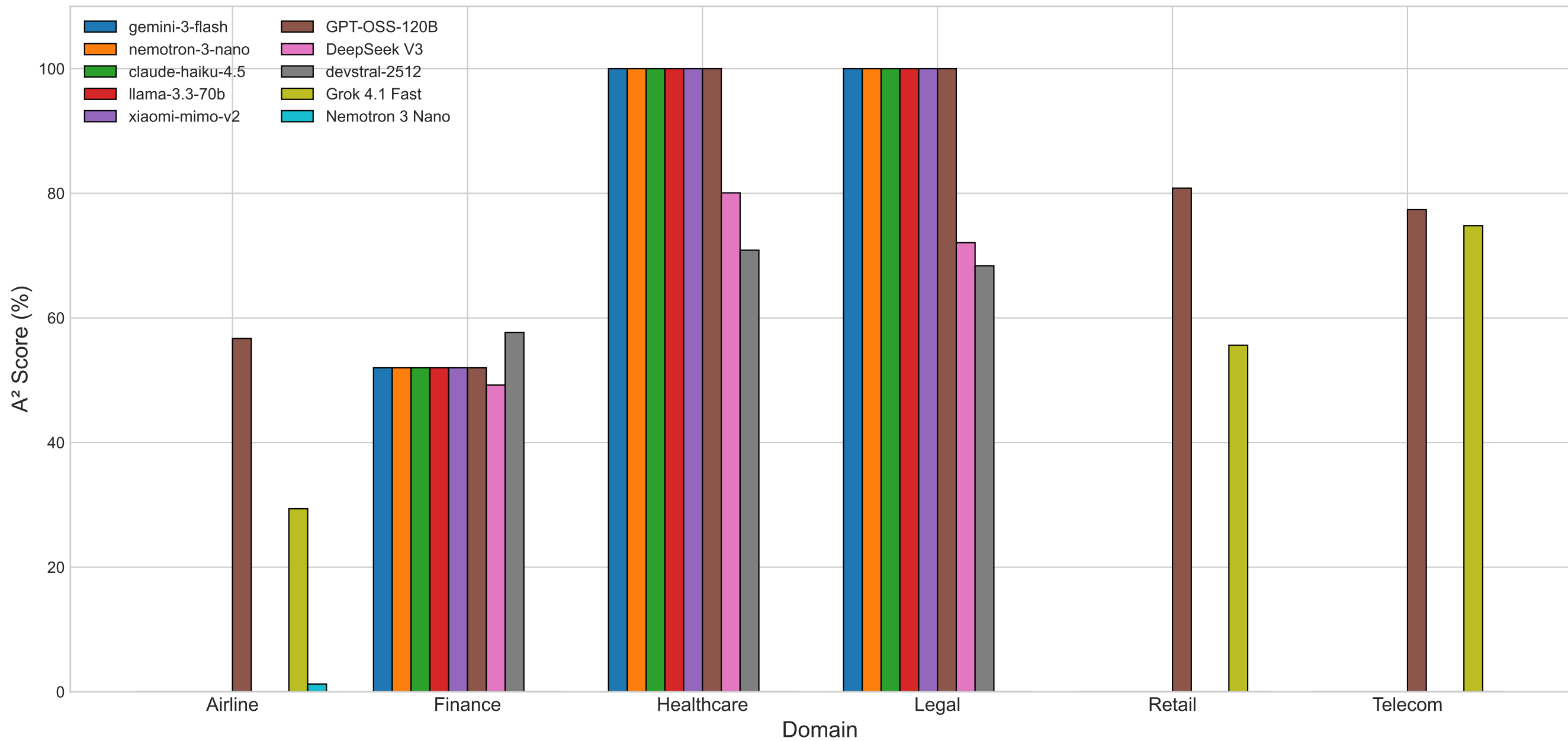
A 2 Scores: Model × Domain
