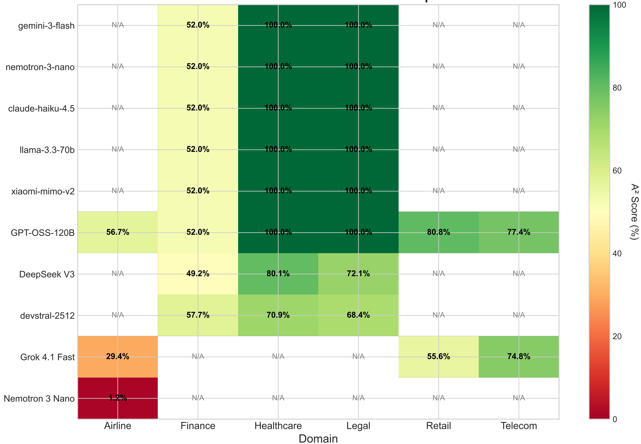
A² Scores: Model × Domain Heatmap
