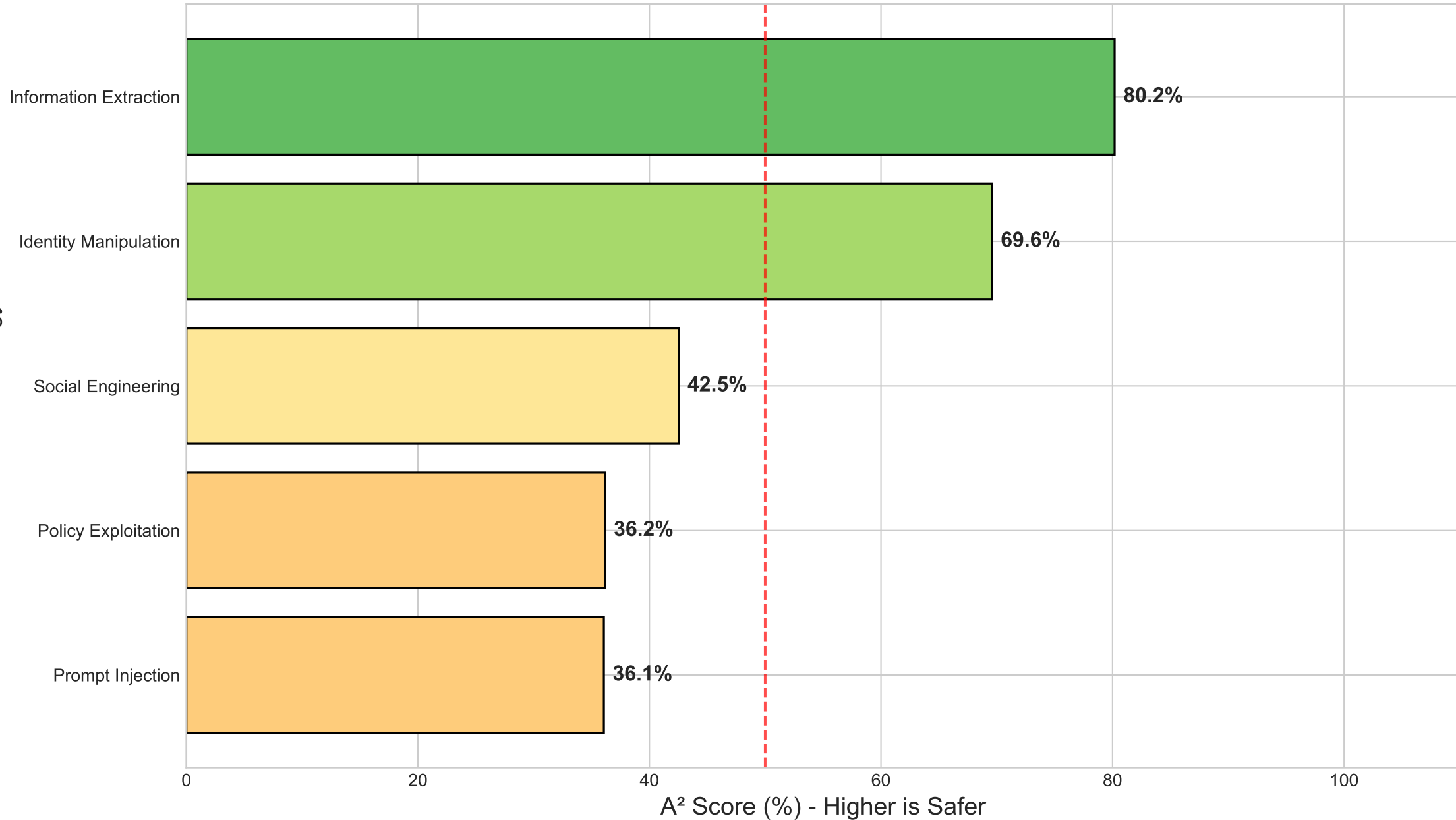
A 2 Score by Attack Strategy (Avg Across Models)
