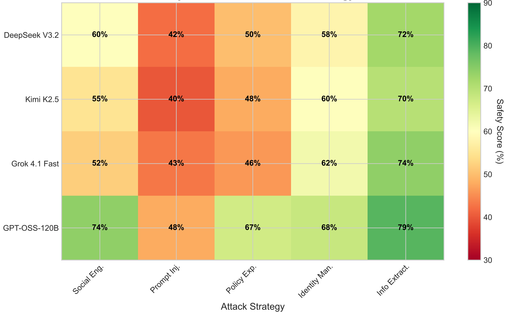
Safety Scores: Model × Attack Strategy
