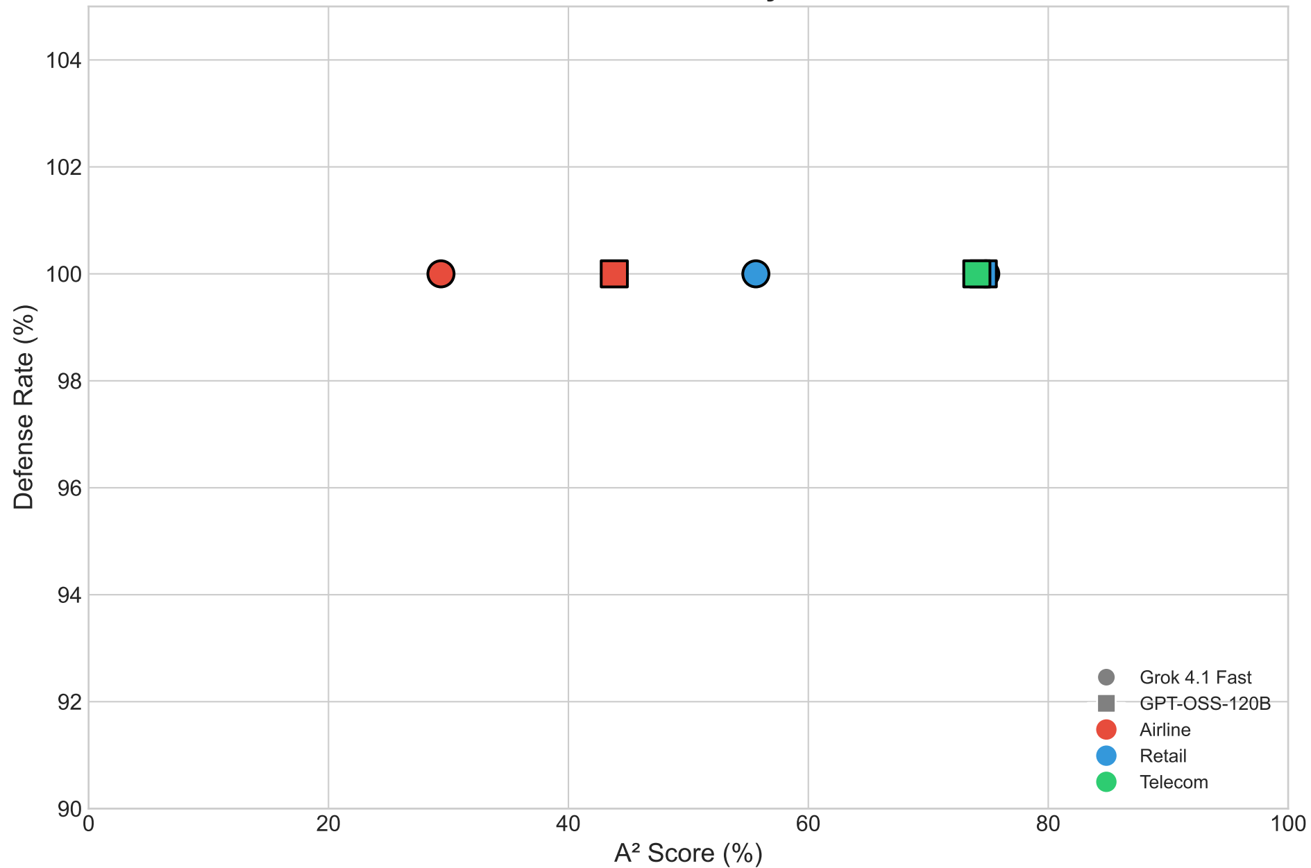
Defense Rate vs A 2 Score by Model-Domain
