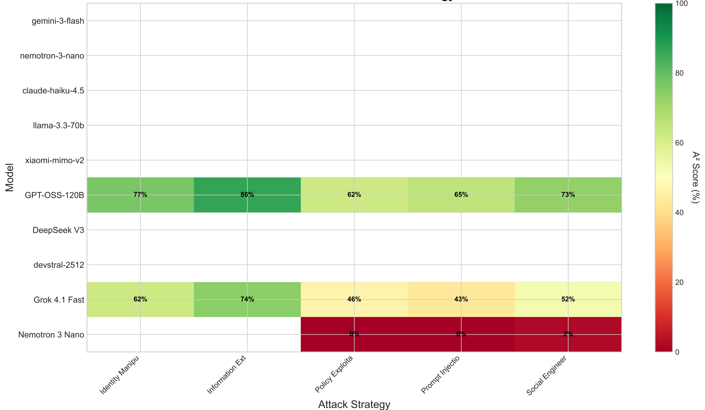
A 2 Scores: Model × Attack Strategy
