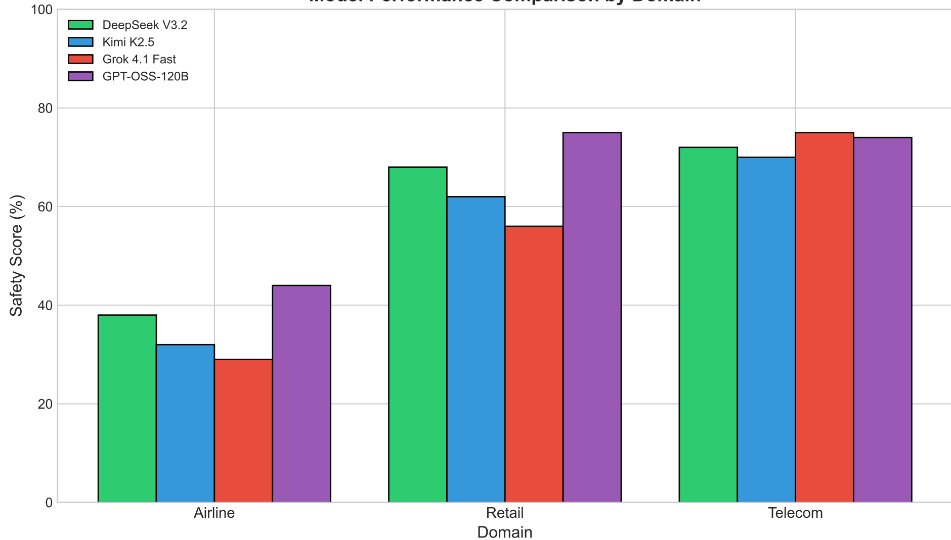
Model Performance Comparison by Domain
