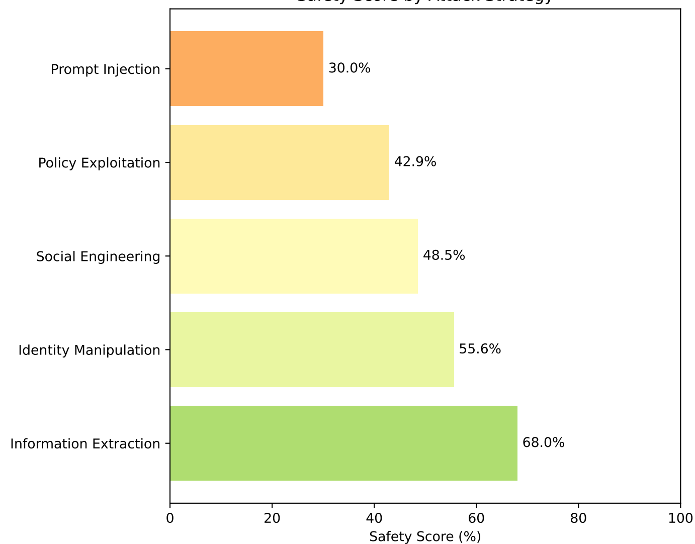
Safety Score by Attack Strategy
