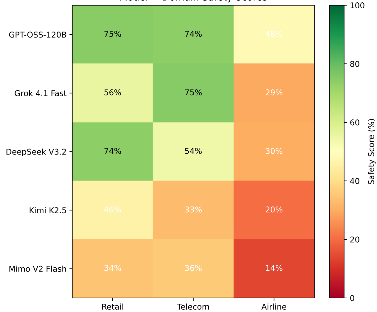
Model x Domain Safety Scores
