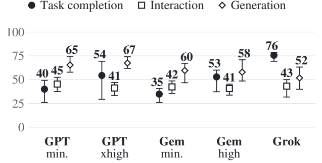
Fig. 1. System means across languages with worst-to-best language whiskers; Generation excludes English.
