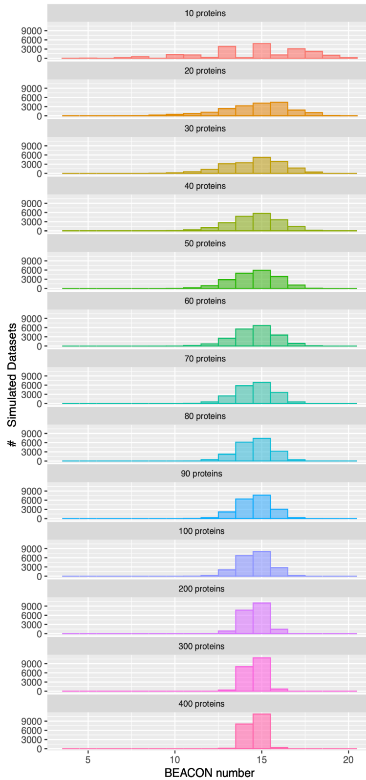
Supplementary Figure 2. Distribution of BEACON numbers for simulated networks of varying size and a medium confidence score show similar means, but shrinking standard deviations as the number of proteins increased.
