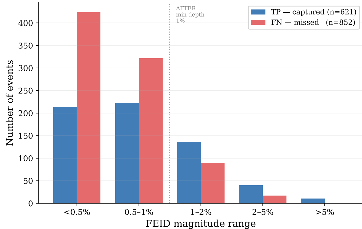
Captured vs missed FEID events by magnitude
