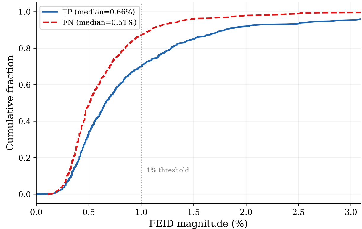
Magnitude CDF: captured vs missed
