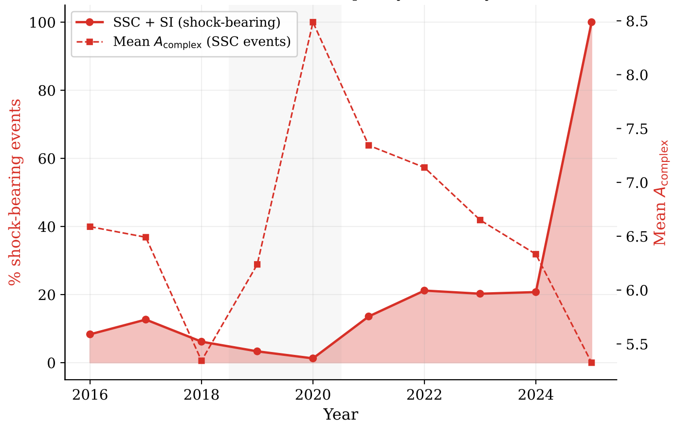
Shock fraction and complexity vs solar cycle
